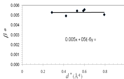
Fig (2) Williamson-Hall plot-TiO 2 nanoparticles
