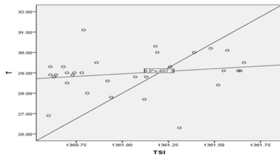
Figure 6. Scatter plot between TSI( Wm^{-2} ) and annual air temperature ( ^{\circ}C ) for the period (1988-2017).
