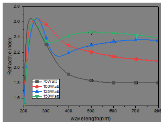
Fig. 6: The refractive index ( n ) as a function of wavelength ( \lambda ) For V_2O_5 thin films deposited at different sputtering power.
