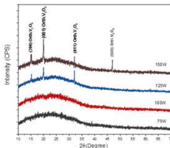
Fig. 1: X-ray diffraction patterns for \text{V}_2\text{O}_5 thin film deposited by different R.F powers
