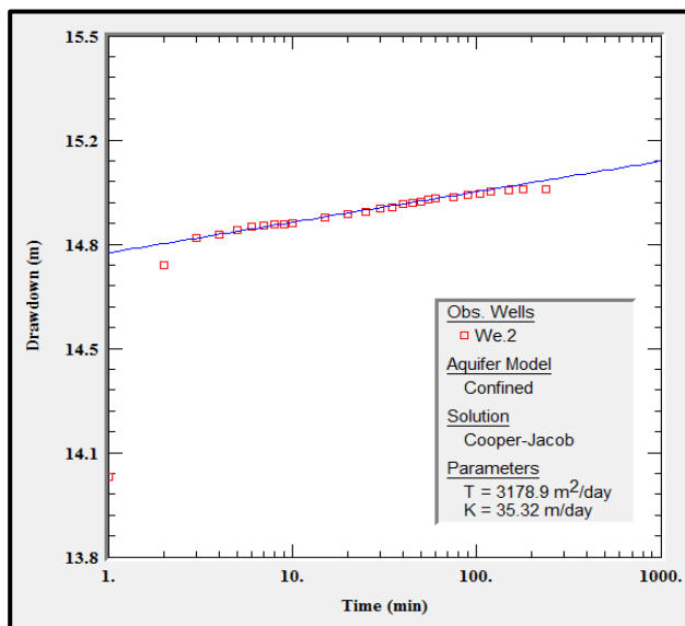
Figure (7): Time-Drawdown curve of well No.2.
