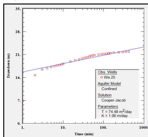
Figure (10): Time-Drawdown curve of well No.25.
