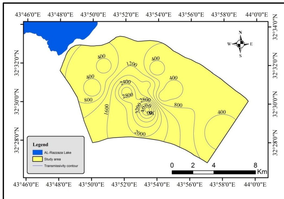
Figure (16): Spatial distribution of the transmissivity values for the aquifer (m 2 /day).
