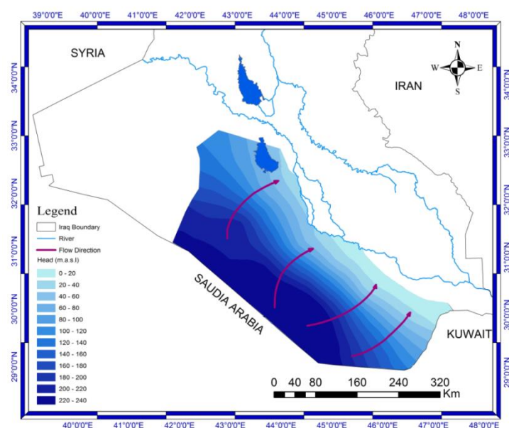
Figure (5): Groundwater movement of the Damman aquifer.
