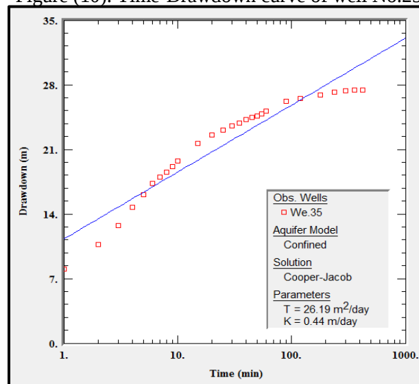
Figure (12): Time-Drawdown curve of well No.35.
