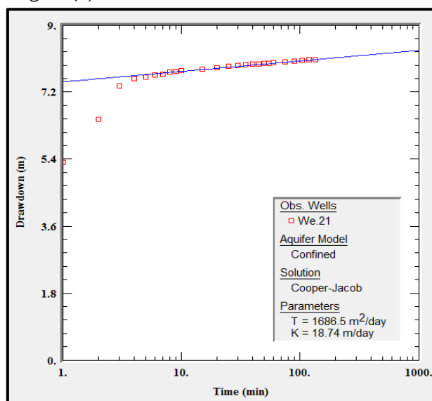
Figure (9): Time-Drawdown curve of well No.21.
