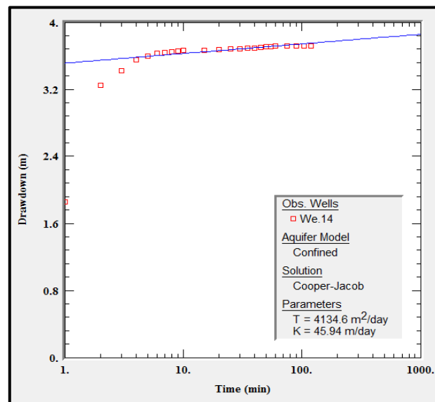
Figure (8): Time-Drawdown curve of well No.14.
