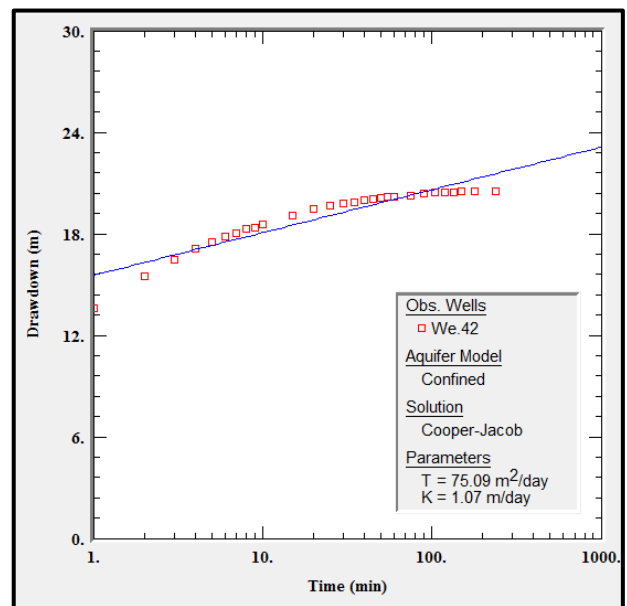
Figure (14): Time-Drawdown curve of well No.42.
