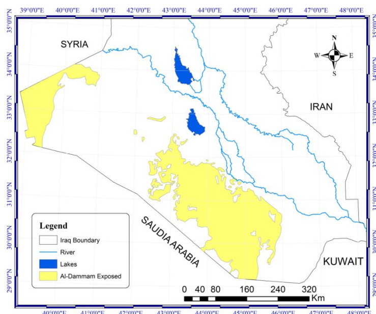
Figure (4): The distribution of Damman outcrop on the surface in desert of Iraq developed from the Geological map of Iraq, 1995.
