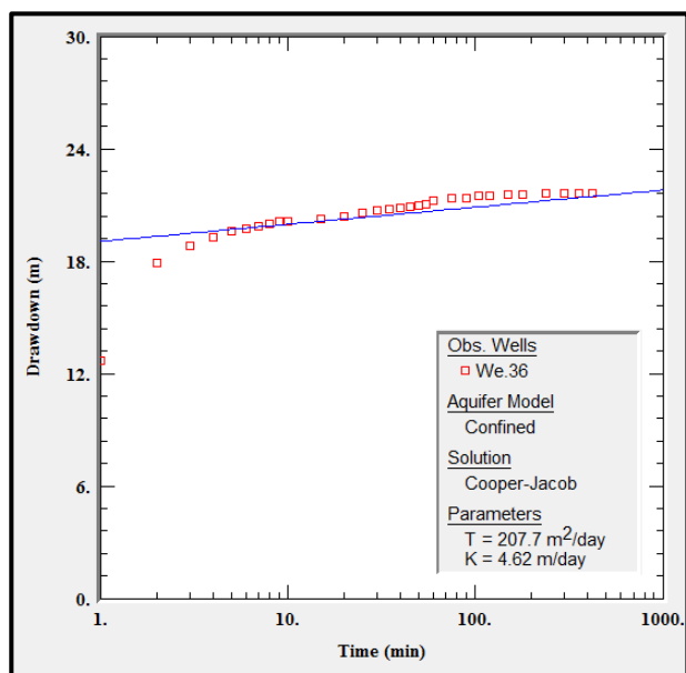
Figure (13): Time-Drawdown curve of well No.36.
