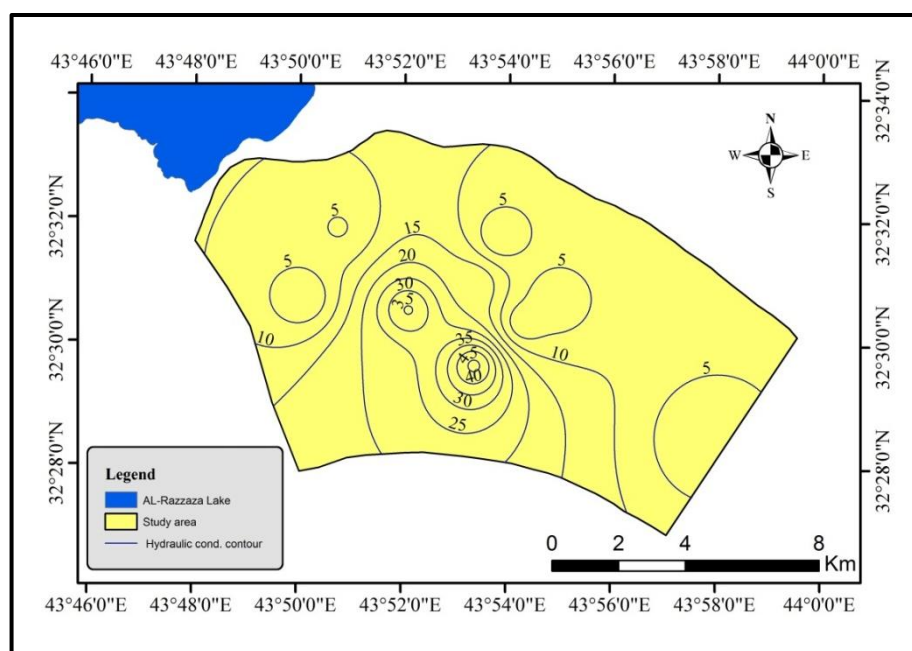
Figure (17): Spatial distribution of the hydraulic conductivity values for the Dammam aquifer (m/day).
