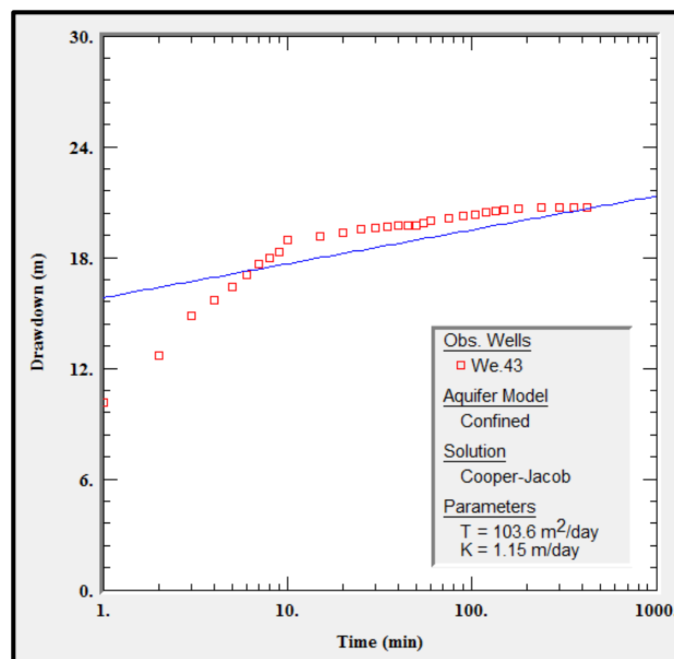
Figure (15): Time-Drawdown curve of well No.43.
