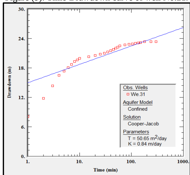
Figure (11): Time-Drawdown curve of well No.31.
