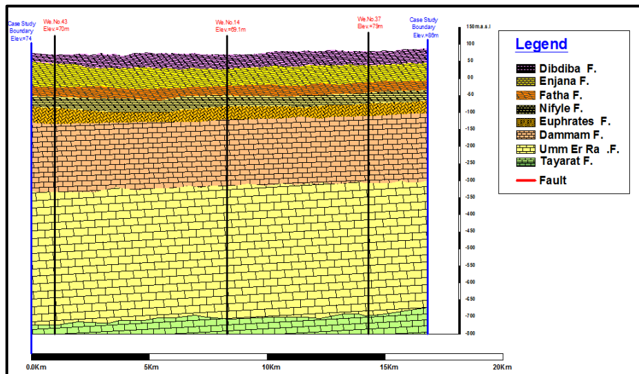
Figure (3): The stratigraphic correlation between the wells in the study area developed from (Consortium, 1977; Sissakian, 1995).
