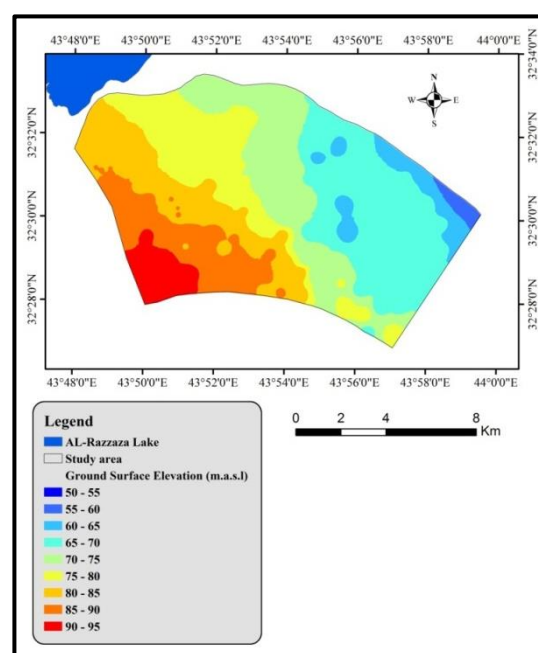
Figure (2): Topography of the study area (after US DEMs).
