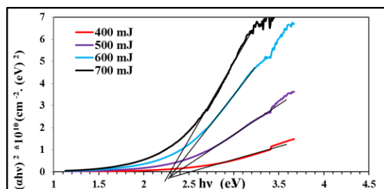
Fig. 8: Variation of (\alpha h\nu)^2 versus photon energy ( h\nu ) for CdO films deposited at different laser energies (400,500,600,700) mJ.
