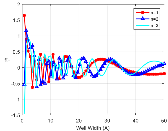
Fig. 6: The eigenfunctions of the ground state ( n=1 ) and the excited states ( n=2,3 ), corresponding to the self-energy states computed using the time-independent Schrödinger equation.
