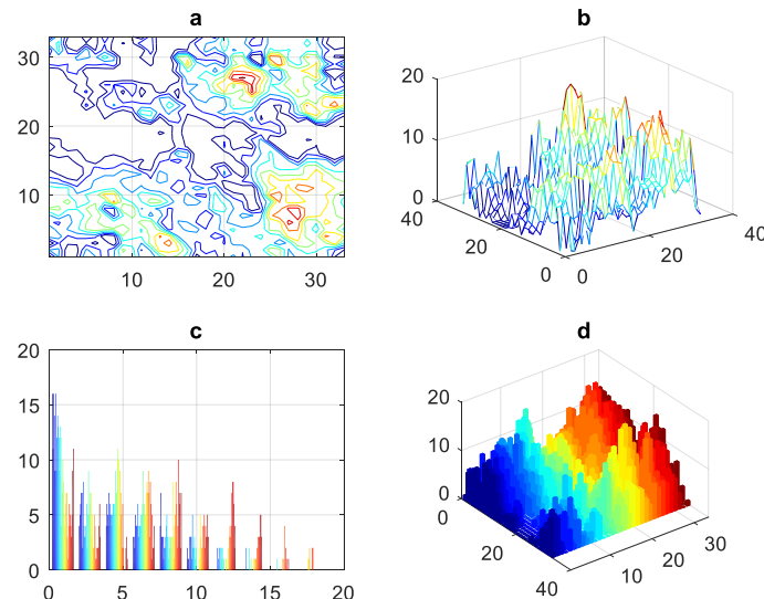
Fig. 2: The localization landscape method: (a) the valley network with blue lines represents the localization limits for the function u , (b) the landscape function u represents the solutions of equation (2), (c) represents a two-dimensional view of the bound states gradient inside the quantum potential well, (d) represents the effective localization potential ( W ) for the sub-regions shown in (a) where W = u^{-1} .
