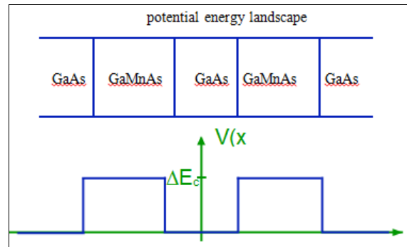
Fig. 1: illustrates a landscape method for the potential energy of a GaAs quantum well, the effective mass was taken in the calculations.
