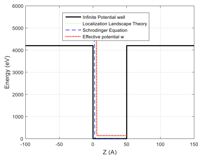
Fig. 3: Shows a comparison between the possibility of quantum confinement and wavefunction localization for the Landscape and Schrodinger method, it is clearly that there is a high congruence in the two methods, as the error rate is approximately 0.1% between the two methods, width of the well is 50 Å with infinite barriers.
