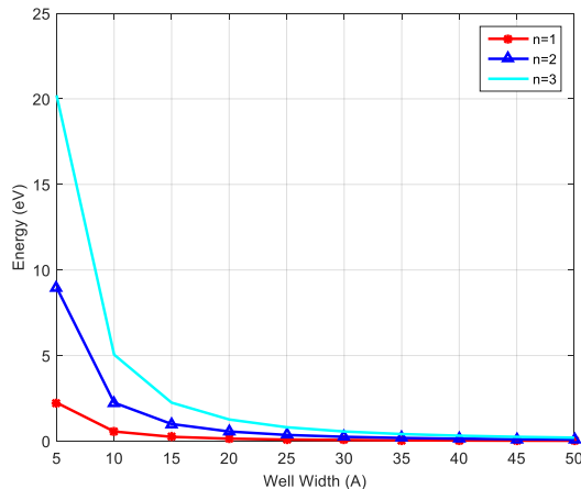
Fig. 4: Shows the lowest three states of energy eigenvalue in a GaAs potential well, width of 50 Å surrounded by infinite barriers. It is clearly that all three states appear coherent with decreasing energy value during increasing the well width.
