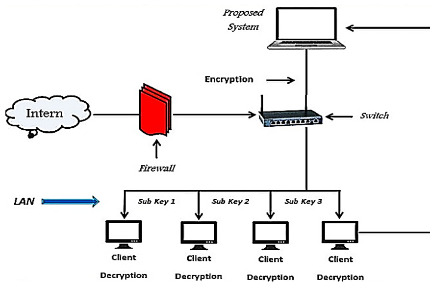
Figure 3: The design of the proposed Simulation RC5 Algorithm based peer to peer (SRPP)
