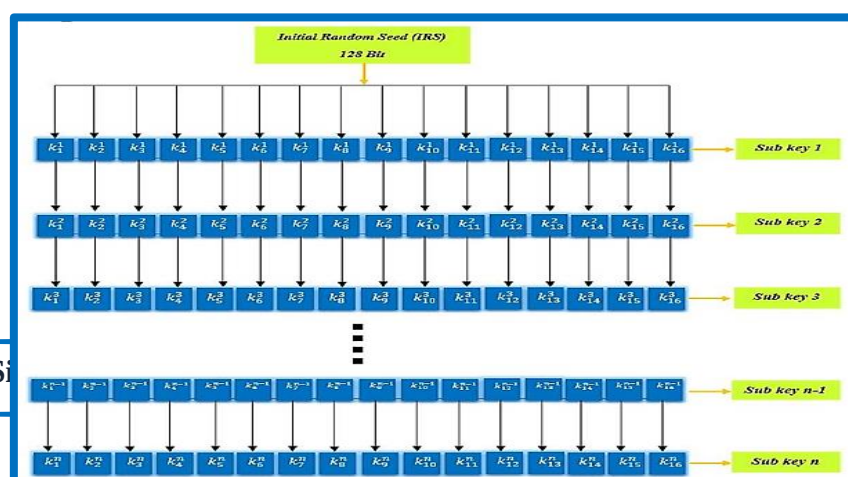
Figure 2: Block diagram of ERC5KS
