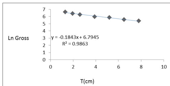
Fig. 9: Relationship between thickness T(cm) and Ln Gross for coincidence measurements of Cu at the 1173keV gate.
