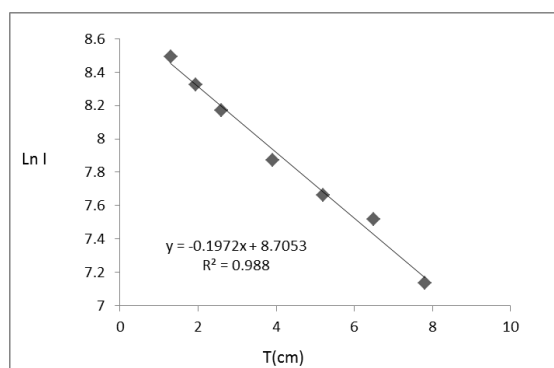
Fig. 7: Relationship between thickness T(cm) and Ln I for direct measurements of Cu at the 1173keV gate.
