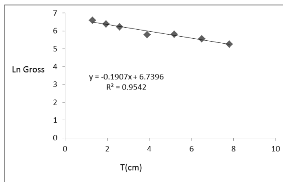
Fig. 6: Relationship between thickness T(cm) and Ln Gross for coincidence measurements of Cu at the 1332keV gate.
