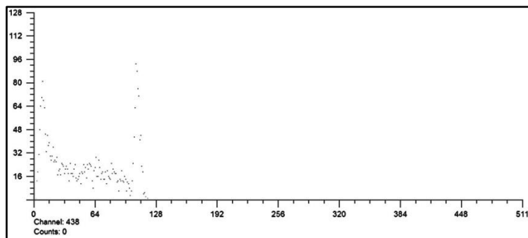
Fig. 8: coincidence Spectrum at the 1173KeV gate.
