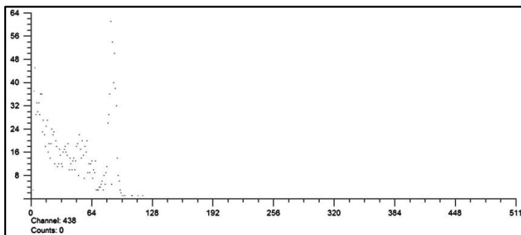
Fig. 5: coincidence Spectrum at the 1332KeV gate.
