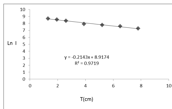
Fig. 4: Relationship between thickness T(cm) and Ln I for direct measurements of Cu at the 1332keV gate.
