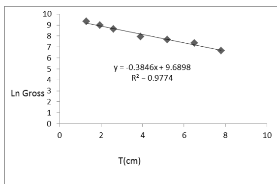
Fig. 3: Relationship between thickness T (cm) and Ln Gross for coincidence measurements of Cu at the 511keV gate.
