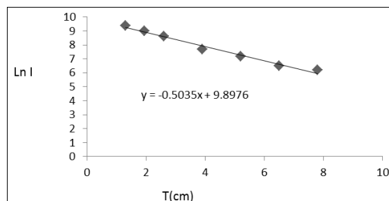
Fig. 2: Relationship between thickness T(cm) and Ln I for direct measurements of Cu at the 511keV gate.
