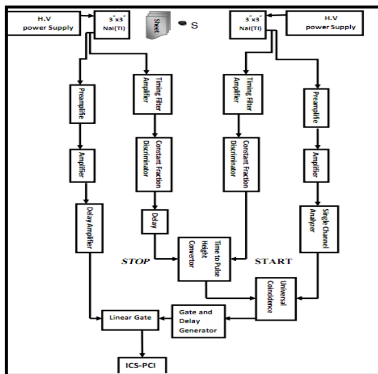
Fig. 1: Block diagram of the gamma-gamma coincidence spectrometer
