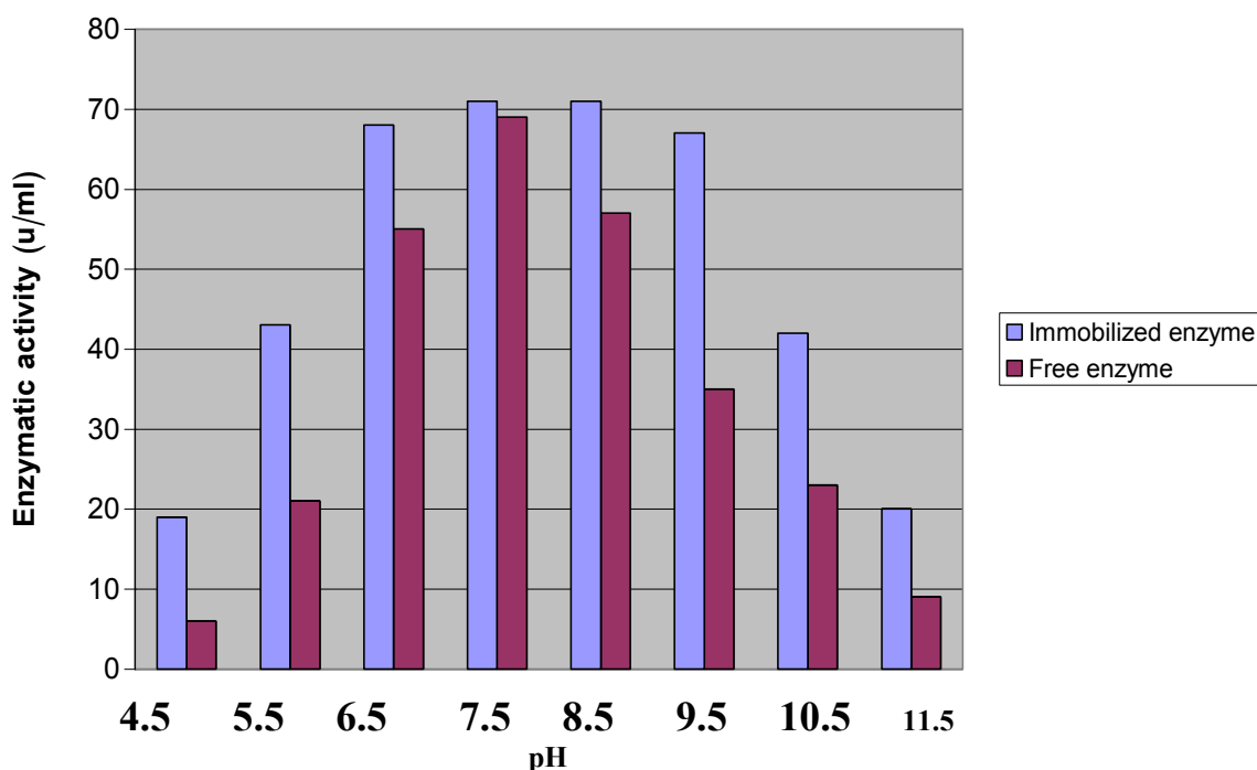
Figure 3. Effect of pH on the activity of free and immobilized cysteine proteinase of E.histolytica
