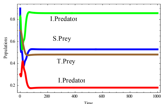
Fig. 7: SI model with harvesting.
