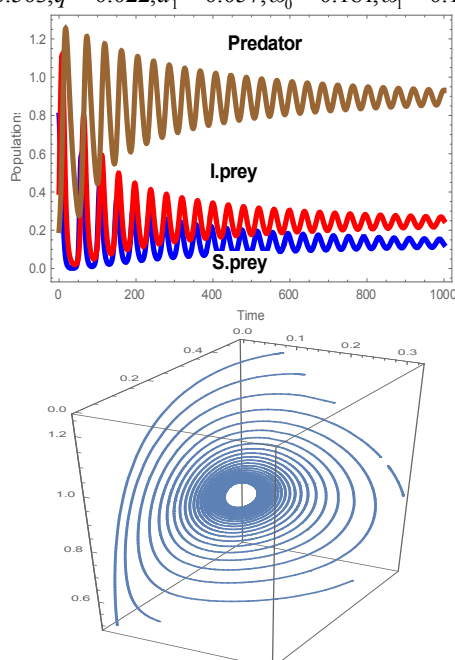
Fig. (5-a) and (5-b): Solution of subsystem (4).
