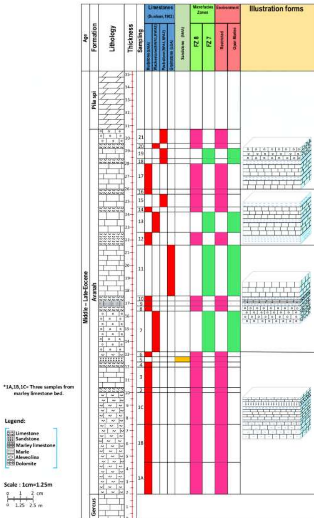
Fig. 2: Environnment distribution of Avanah Formation at the Geli Bessri section Dohuk.
