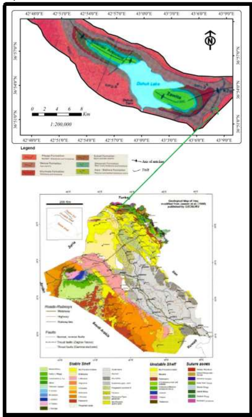
Fig. 1: Geological map of Iraq[7].
