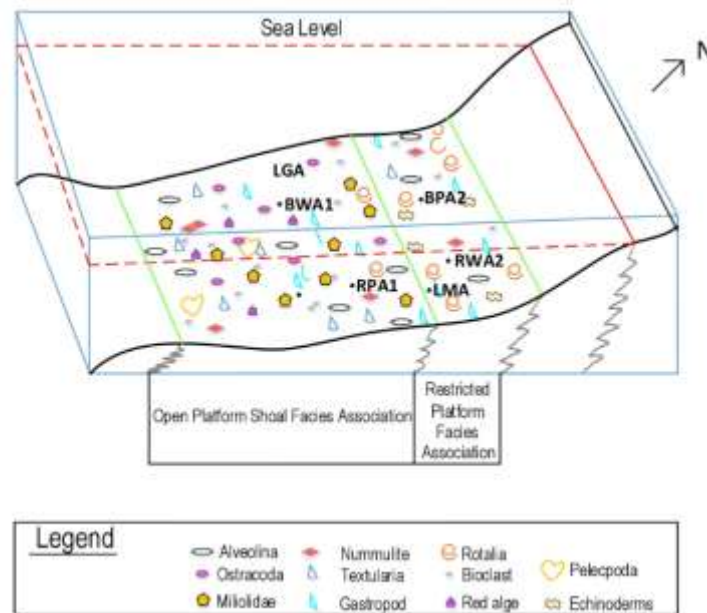
Fig. 3: Depositional model of Avanah Formation.
