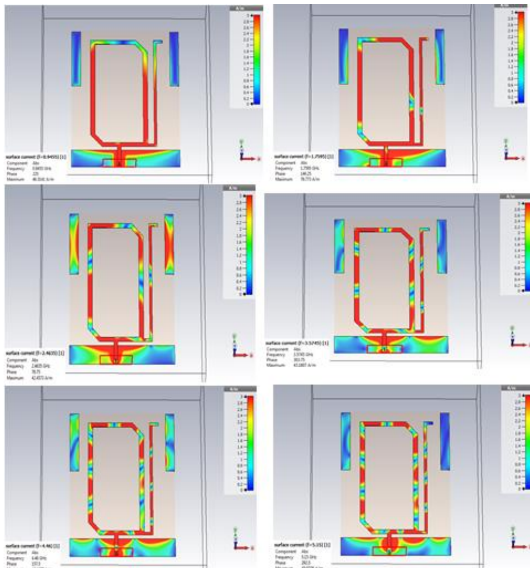
Fig. 8: Current distribution
