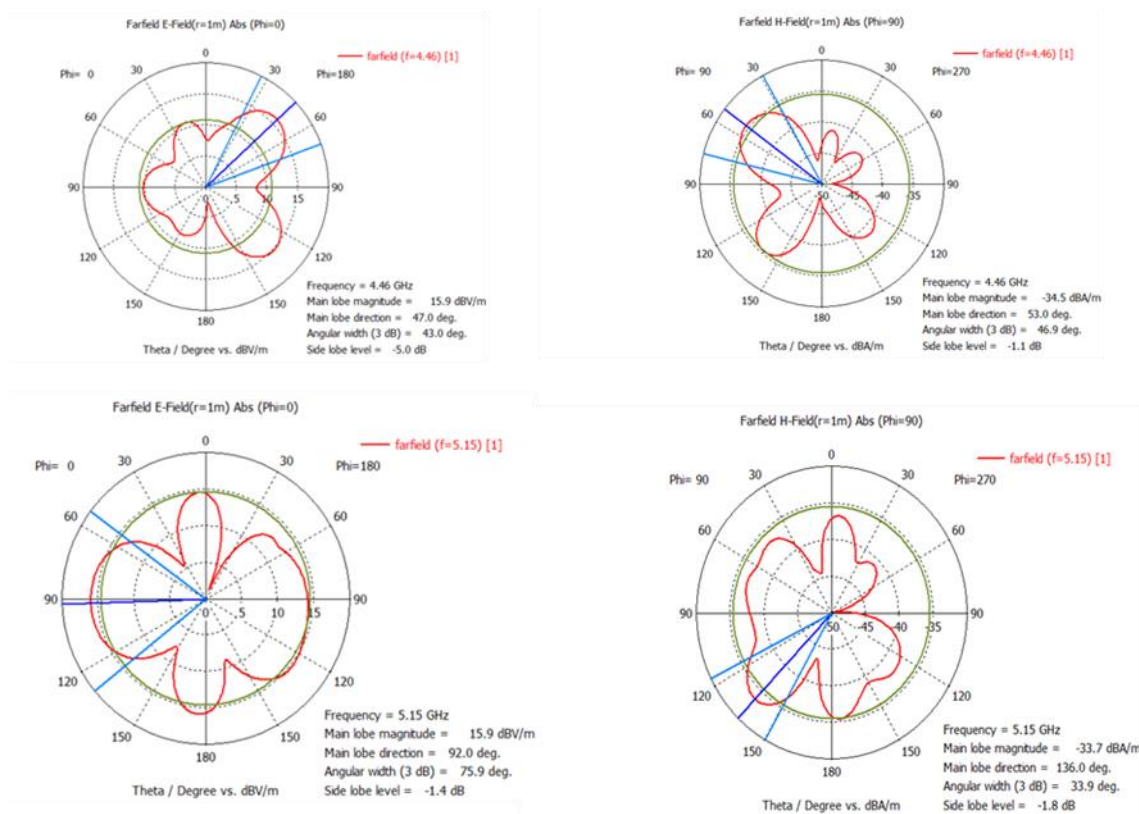
Fig. 7: Radiation pattern
