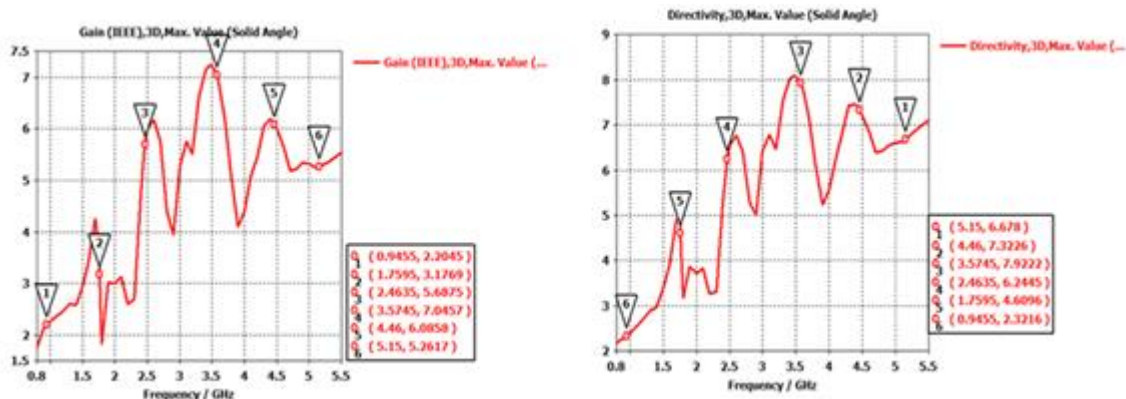
Fig. 5: gain and directivity
