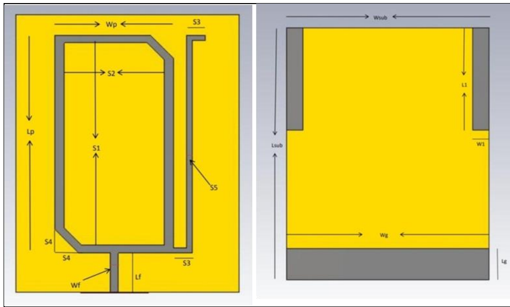
Fig. 2: Structure of the proposed Antenna
