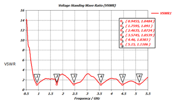
Fig.4: VSWR
