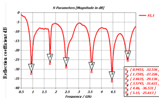
Fig. 3: Reflection coefficient
