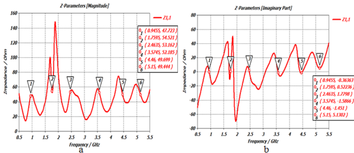
a- Real part b- imaginary part Fig. 6: Impedance versus frequency
