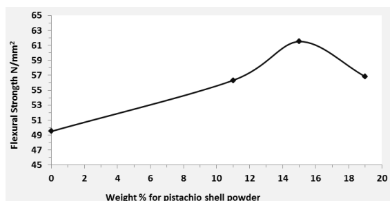
Fig. 10: Pistachio shell particle content versus flexural strength
