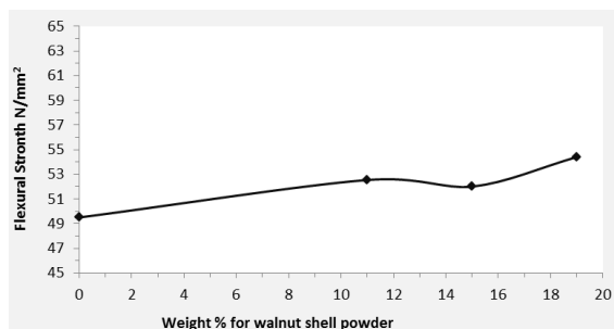
Fig. 9: walnut shell particle content versus flexural strength
