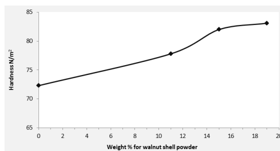
Fig. 7: walnut shell particle content versus hardness
