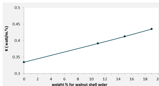
Fig. 11: walnut shell particle content versus thermal conductivity
