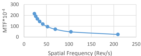
Fig.(14)spatial frequency with MTF at different times and radius (1.5cm)
