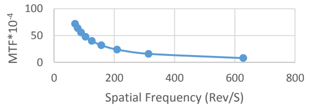
Fig.(17)spatial frequency versus MTF at different radius and time (0.5cm)
