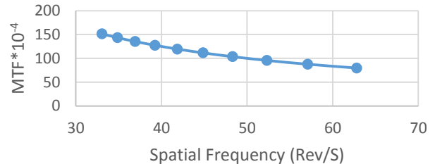
Fig.(18)spatial frequency versus MTF at different radius and time (0.5cm)
