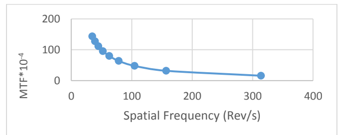
Fig.(12)spatial frequency with MTF at different times and radius (1cm)
