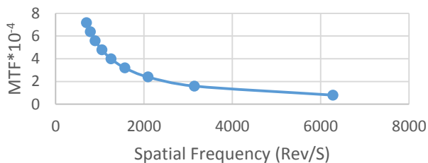
Fig.(15)spatial frequency versus MTF at different radius and time (0.05cm)
