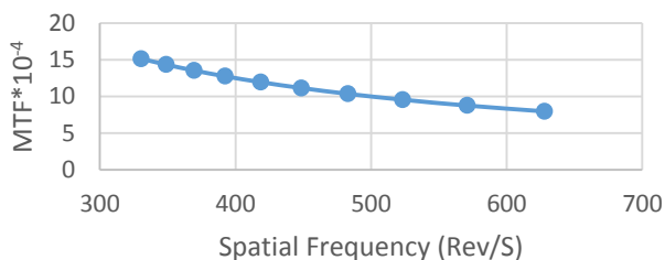
Fig.(16)spatial frequency versus MTF at different radius and time (0.05cm)
