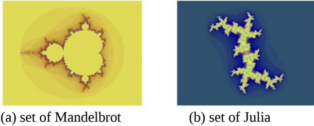
Fig. (3): sets of Mandelbort and Julia
