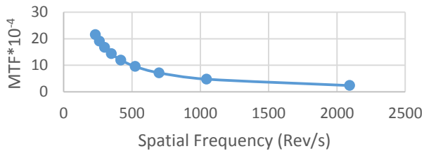
Fig.(13)spatial frequency with MTF at different times and radius (1.5cm)
