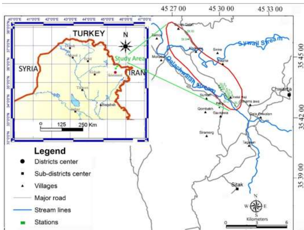
Fig. 1: Topographic map showing the locations of the 10 slope sites in Red bed series in the study area
