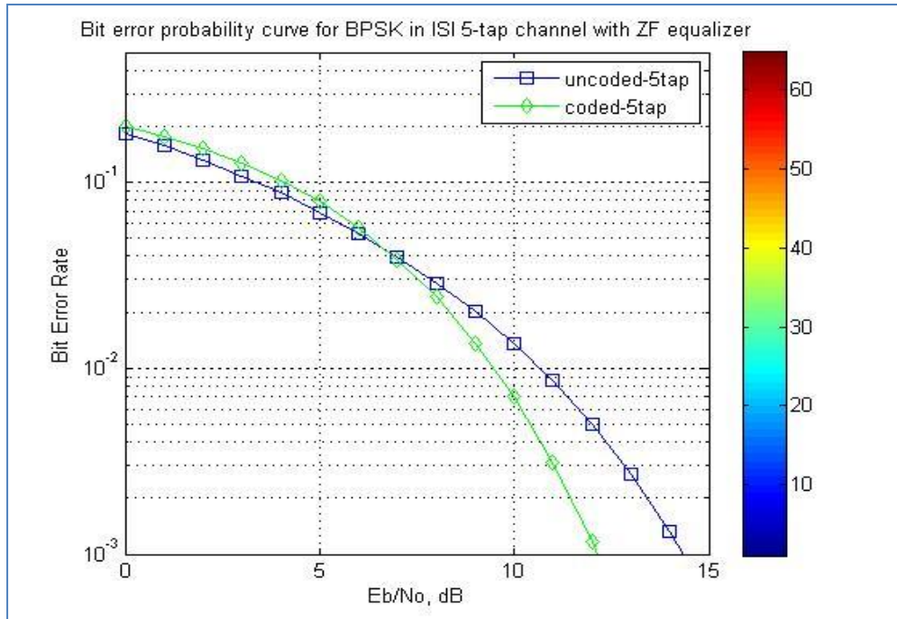
Figure (6): Bit error probability curve for BPSK in ISI channel with ZF equalizer using Systematic Hamming code (31,26)
