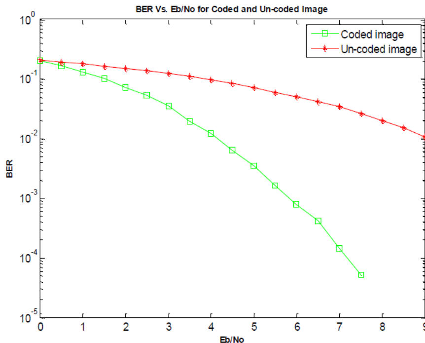
Figure (3): BER versus E_b/N_0 for coded and Un-coded image
