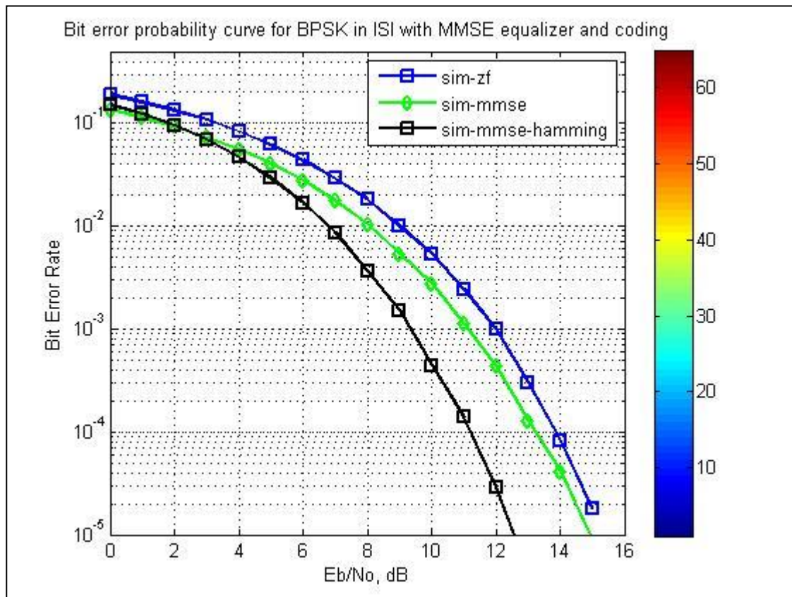
Figure (5): BER curve for BPSK in ISI channel with MMSE equalizer using Systematic Hamming code (15,11)
