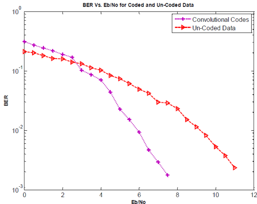
Figure (2): BER (bit error rate) versus E_b/N_0 for Un-coded and coded data
