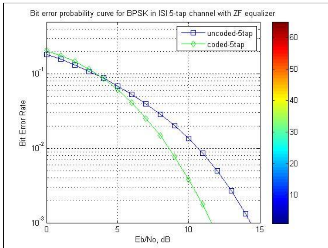
Figure (4) Bit error probability curve for BPSK in ISI channel with ZF equalizer using Systematic Hamming code (15,11)
