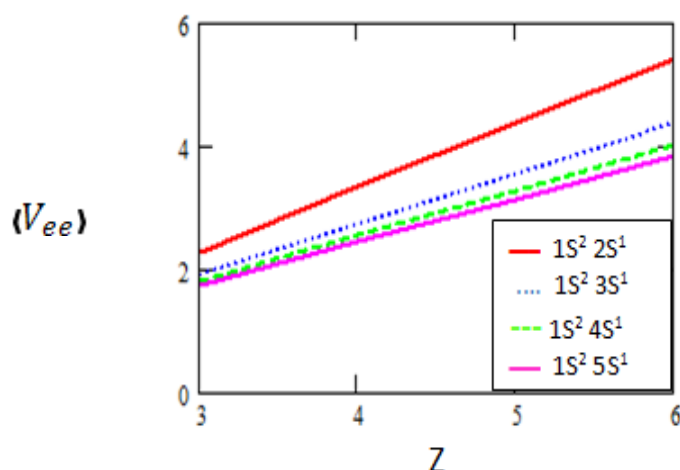
Figure (1) shows the relation between \langle V_{ee} \rangle versus z of (1s^2 2s^1) , (1s^2 3s^1) , (1s^2 4s^1) and (1s^2 5s^1) configurations.
