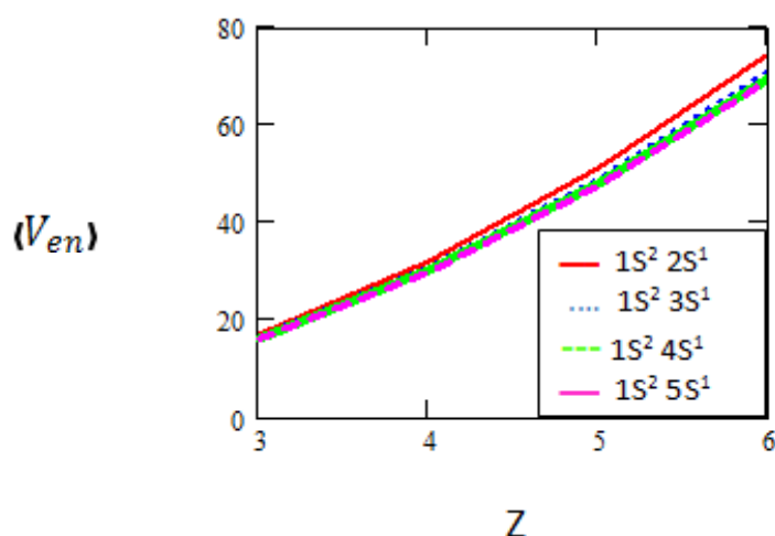
Figure (2) shows the relation between \langle V_{en} \rangle versus z of (1s^2 2s^1) , (1s^2 3s^1) , (1s^2 4s^1) and (1s^2 5s^1) configurations.
