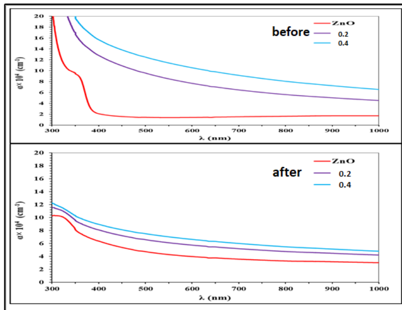
Fig. 7: absorption coefficient before and after annealing
