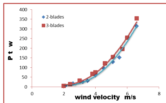
Fig 8: Relation between wind velocity and power turbine
