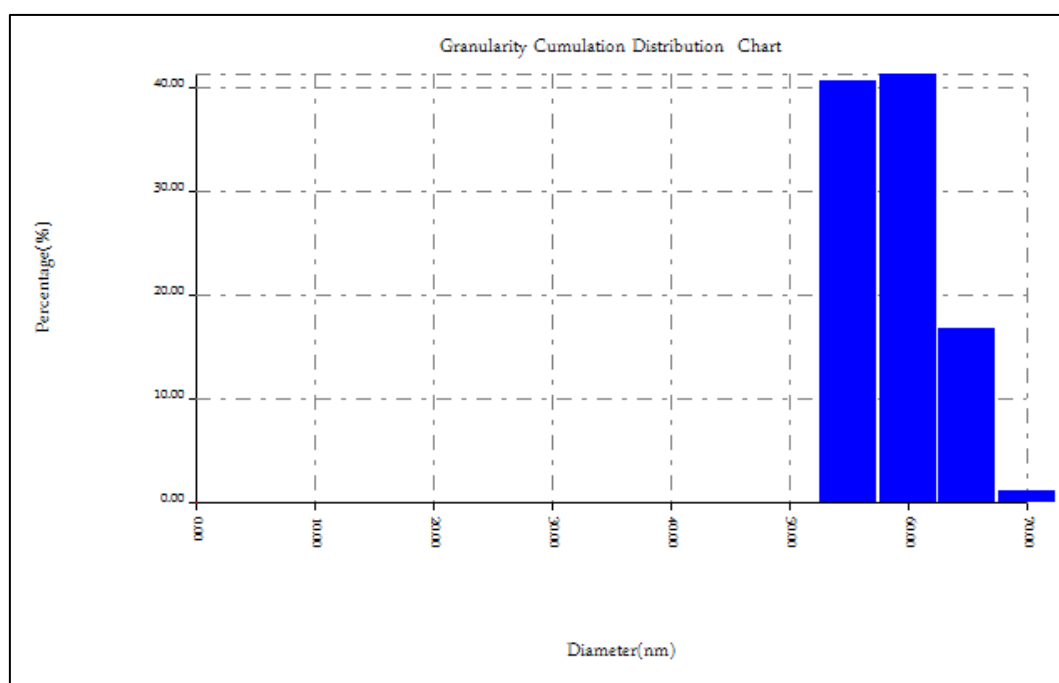
Fig. 4: represents a graph of the granular groups distribution percentages on the surface of the pressed \text{AgNO}_3 sample.
