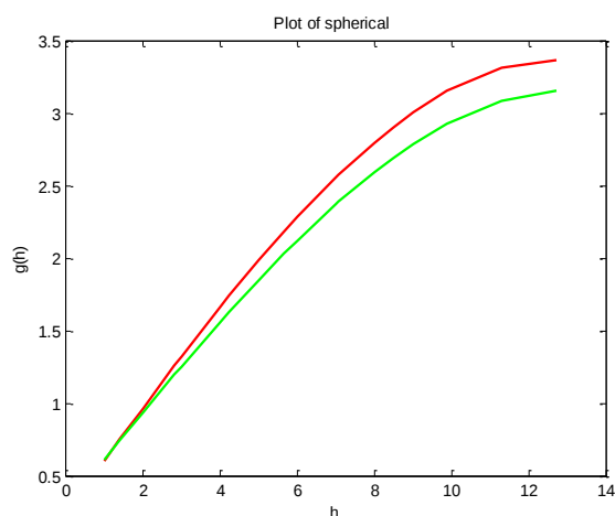
Fig. 3: is the best estimate of the spherical model
