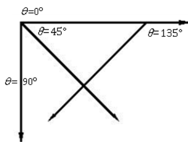
Fig. 1: The four angles used to calculate the semi-variogram function represent the indicator
