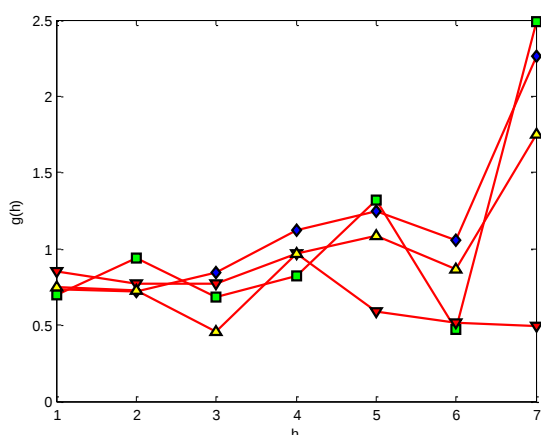
Fig. 2: The semi-variogram Indicator at the four corners, which shows it as a beam indicating the isotropic property.
