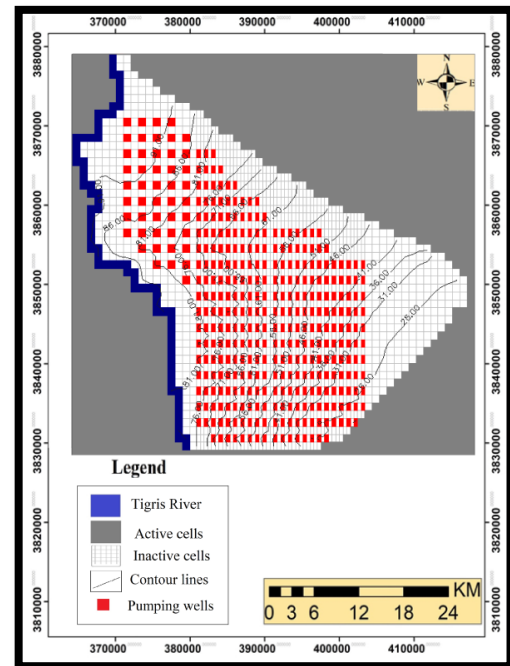
Fig. 8: Water table when drilling 400 wells and pumping (54432 m 3 / year) for each well
