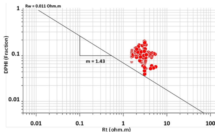
Fig. 13: Pickett's crossplot for estimation of cementation exponent ( m ) for the studied Ibrahim Formation in the well H-1.
