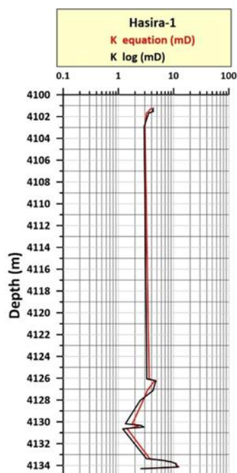
Fig. 9: Matching between the measured permeability from equation and from MLR method for the studied Ibrahim Formation in the well H-1.
