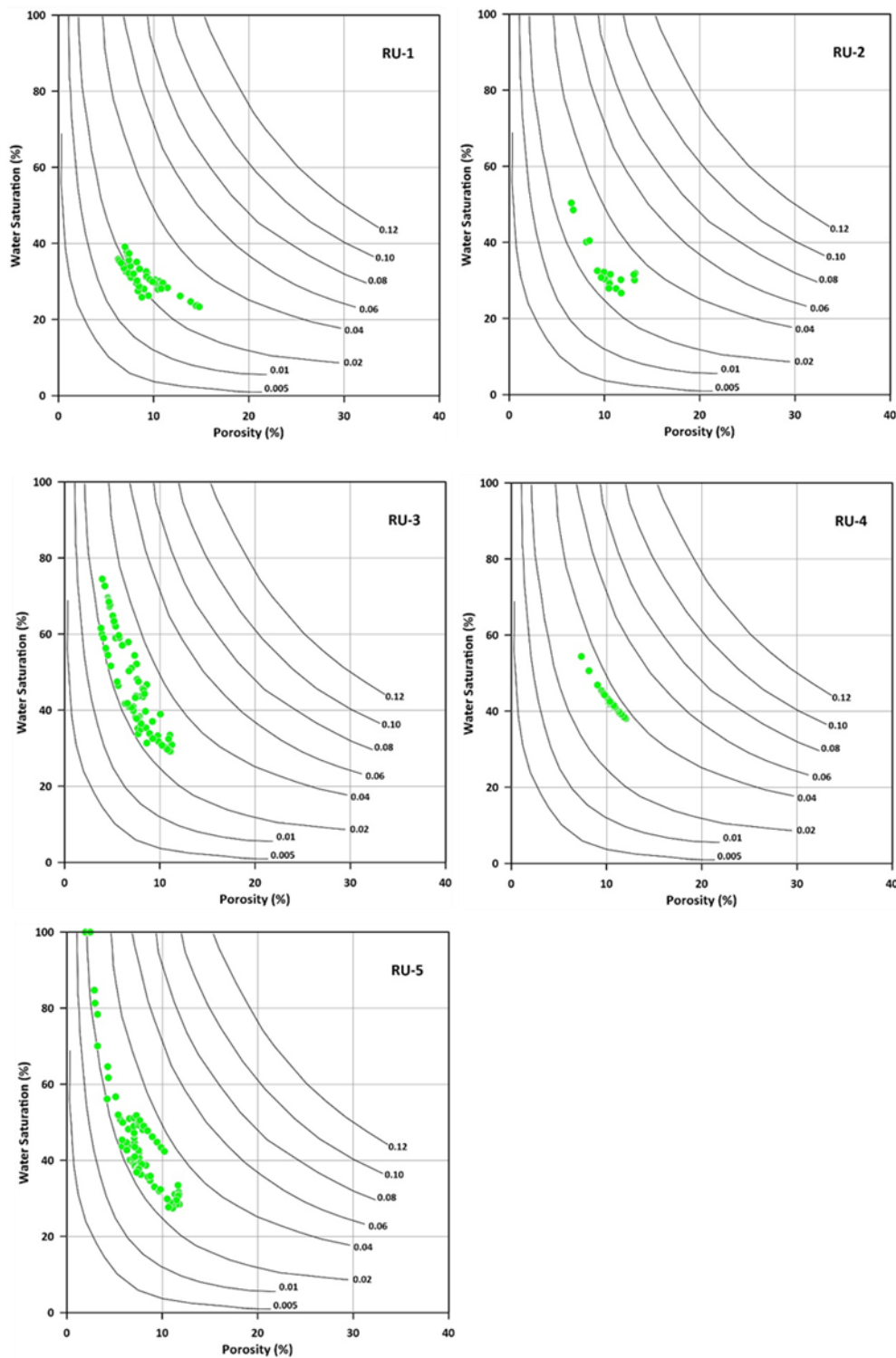
Fig. 15: Buckles plot for the BVW values of the reservoir units of the Ibrahim Formation in the studied well H-1.
