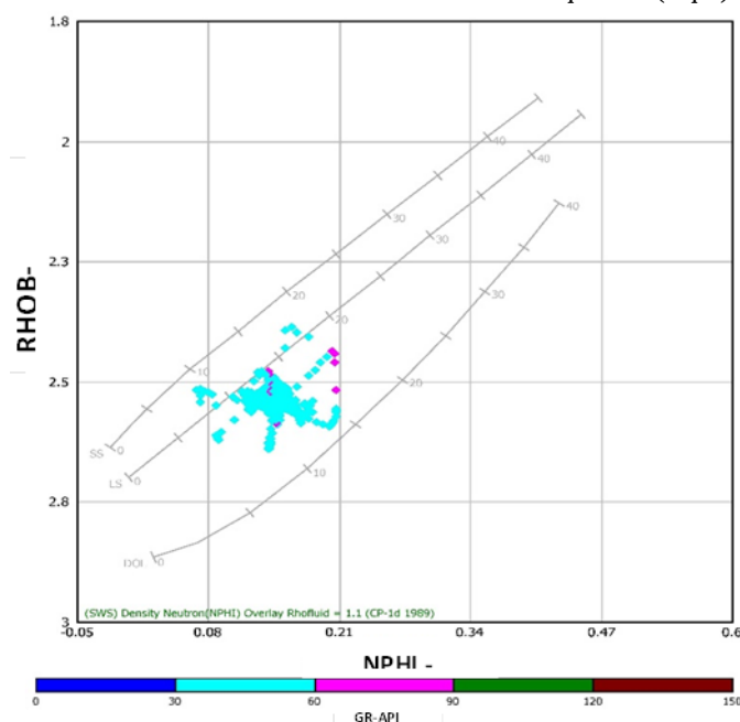
Fig. 5: Lithology identification from N-D crossplot for the Ibrahim Formation in the well H-1 (The crossplot is after [26]).
