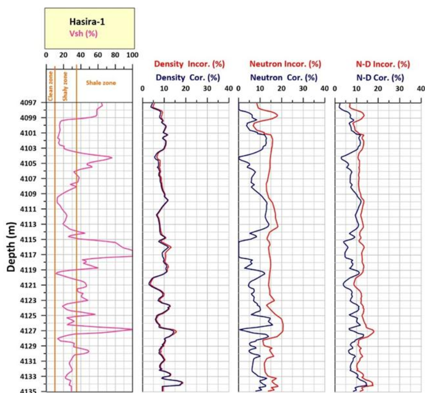
Fig. 7: Shale content and the incorrect and corrected porosities from shale effect for the studied Ibrahim Formation in the well H-1.
