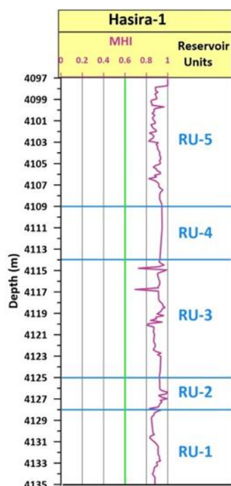
Fig. 16: Movable Hydrocarbon Index for the studied Ibrahim Formation in the well H-1.
