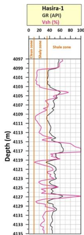
Fig. 6: The record of the Gamma-ray log and the calculated volume of shale for the Ibrahim Formation in the well H-1.
