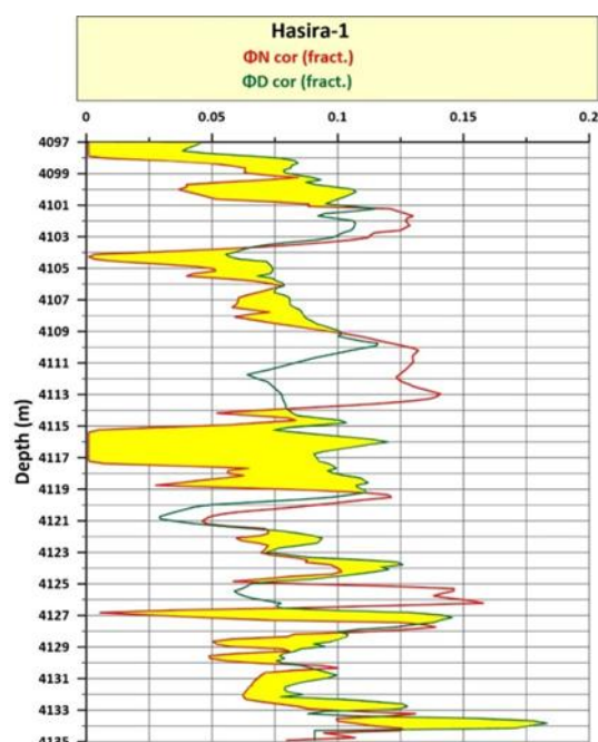
Fig. 8: Crossover of Neutron and Density porosity curves for the Ibrahim Formation in the well H-1.
