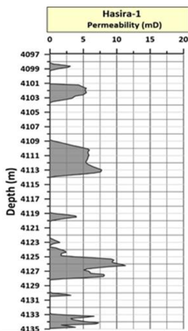
Fig. 10: Calculated permeability from log data for the studied Ibrahim Formation in the well H-1.
