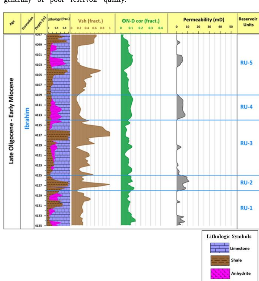
Figure 11: Division of Ibrahim Formation into reservoir units on the bases of variations in shale content, porosity, and permeability in the well H-1.
