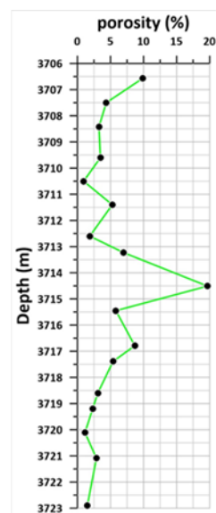
Fig. 17: Curve plot of the measured porosity for the studied Ibrahim Formation in Taza-3 well.
