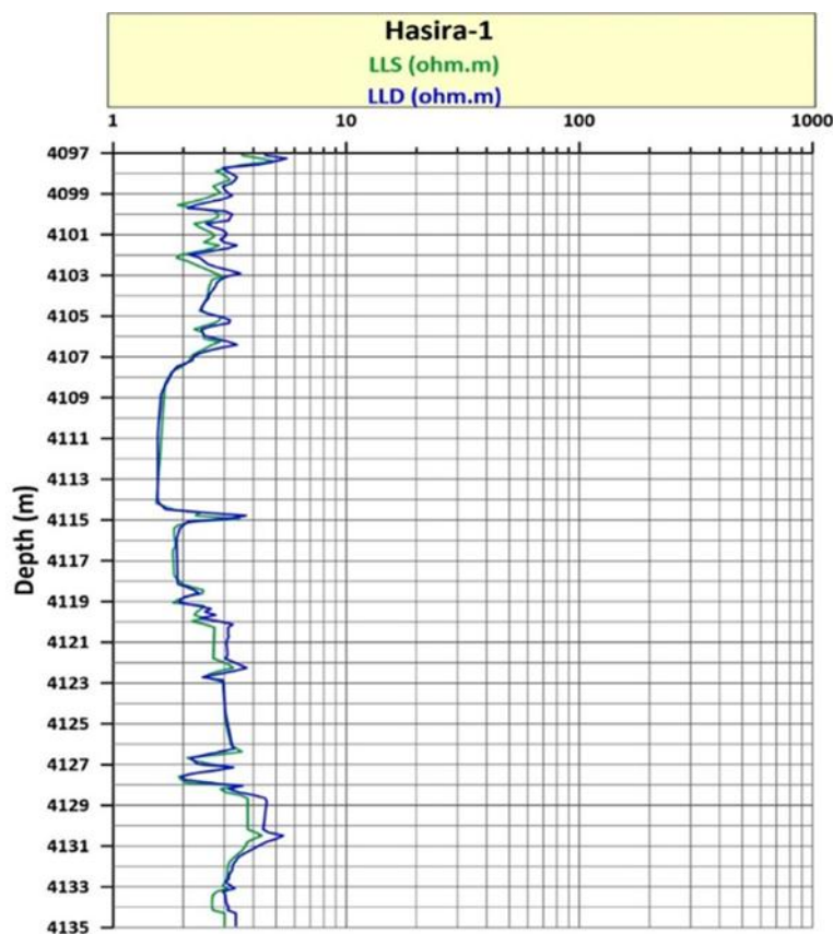
Fig. 12: The recorded LLS and LLD logs for the Ibrahim Formation in the studied well H-1.
