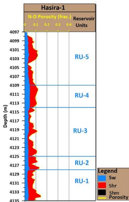
Figures 14: Water saturation and hydrocarbon saturation (residual and movable) with regard to porosity for the studied Ibrahim Formation in the well H-1.
