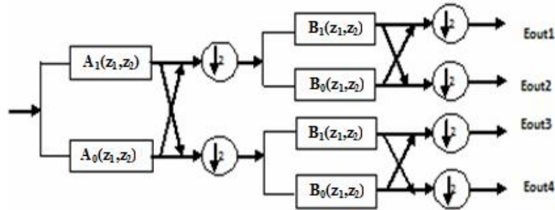
(b) 4-band (DBF) of the contourlet transformation analysis bank.
