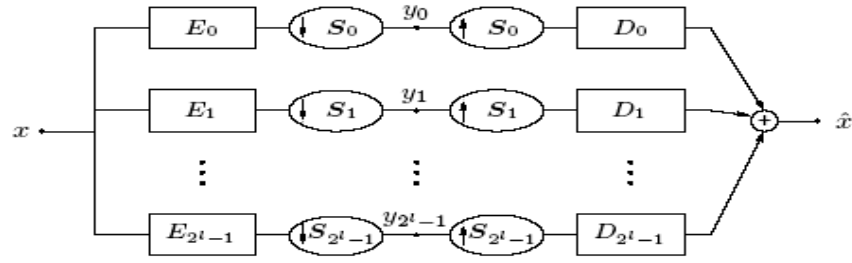
(c) The multichannel view of a one level tree-structured DFB, E_i 's, ( i=0,1,2,\dots, 2^{l-1} ), are the analysis filter functions, D_i 's, ( i=0,1,2,\dots, 2^{l-1} ), are the synthesis filter functions, and S_i 's, ( i=0,1,2,\dots, 2^{l-1} ), are either the down- or up- samplers.
