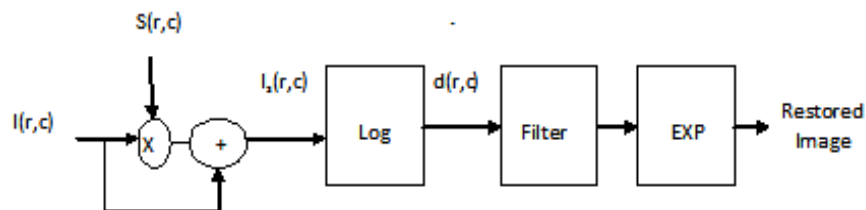
Fig. 1 A signal flow diagram of a typical homomorphic transformation.
