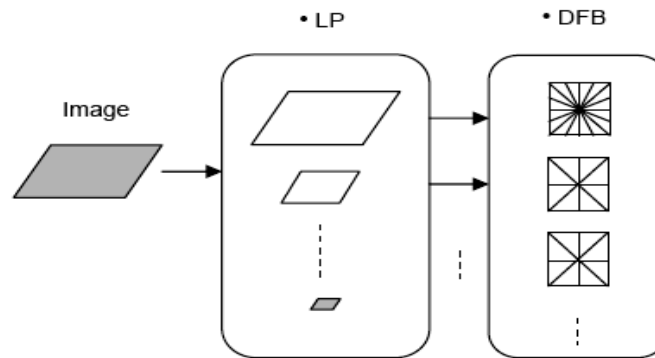
Fig. 2 A flow graph of the contourlet transform. Image is first decomposed into subbands by LP and then each detail image is analyzed by DFB.
