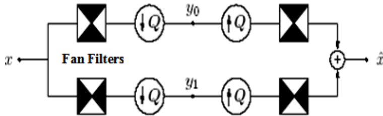
(b) 2-D spectrum partition using quincunx filter banks with fan filters.
