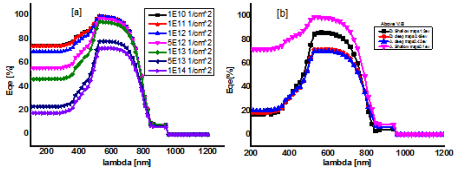
Fig. 3: shows the change of quantum characteristics with change [a] The density of the states of interface defects and [b] the location of the energy level of the defects.
