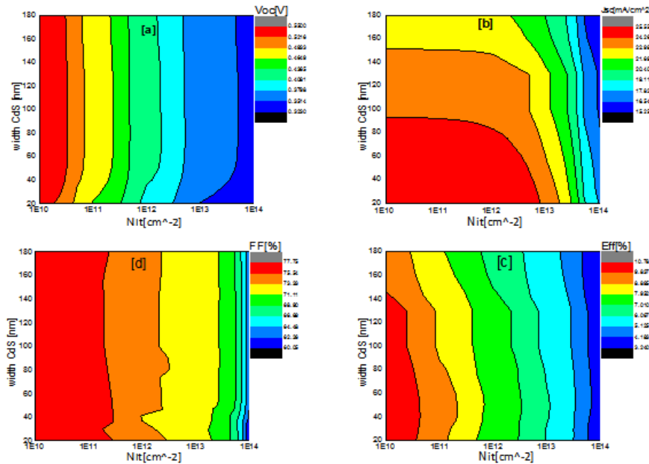
Fig. 7: illustrates the effect of buffer layer thickness and interface density on the performance of the solar cell.
