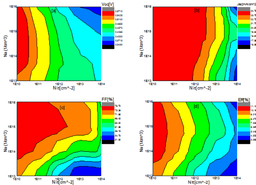
Fig. 9: shows the effect of the concentration of N_A impurities with the density of the interface states on the performance of the solar cell
