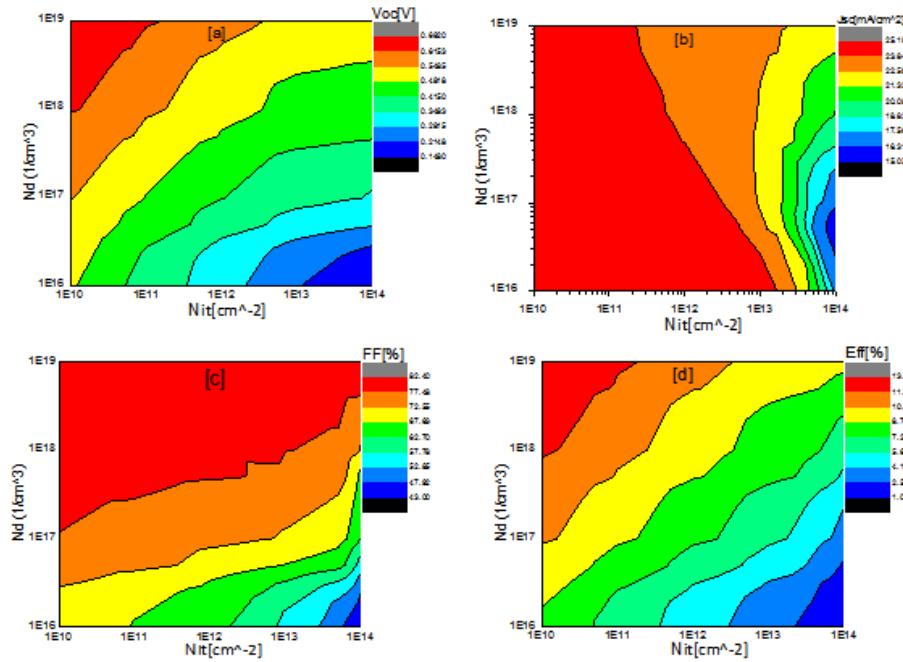
Fig. 11: shows the effect of the concentration of N_D impurities with the density of the interface states on the performance of the solar cell
