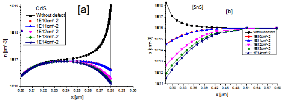
Fig. 4: shows the change in the concentration of charge carriers [a] electrons and [b] holes with the change in the density of the interface states
