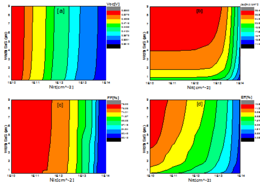
Fig. 5: shows the effect of the thickness of the absorption layer with the density of the interface states on the performance of the solar cell
