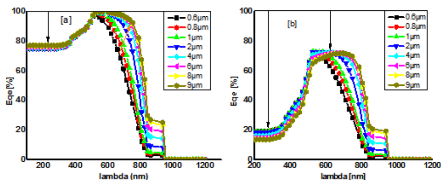
Fig. 6: shows the change of quantum efficiency at the density of the interface states[a] 1E10 \text{ cm}^{-2} and [b] 1E14 \text{ cm}^{-2} with the change in SnS thickness.
