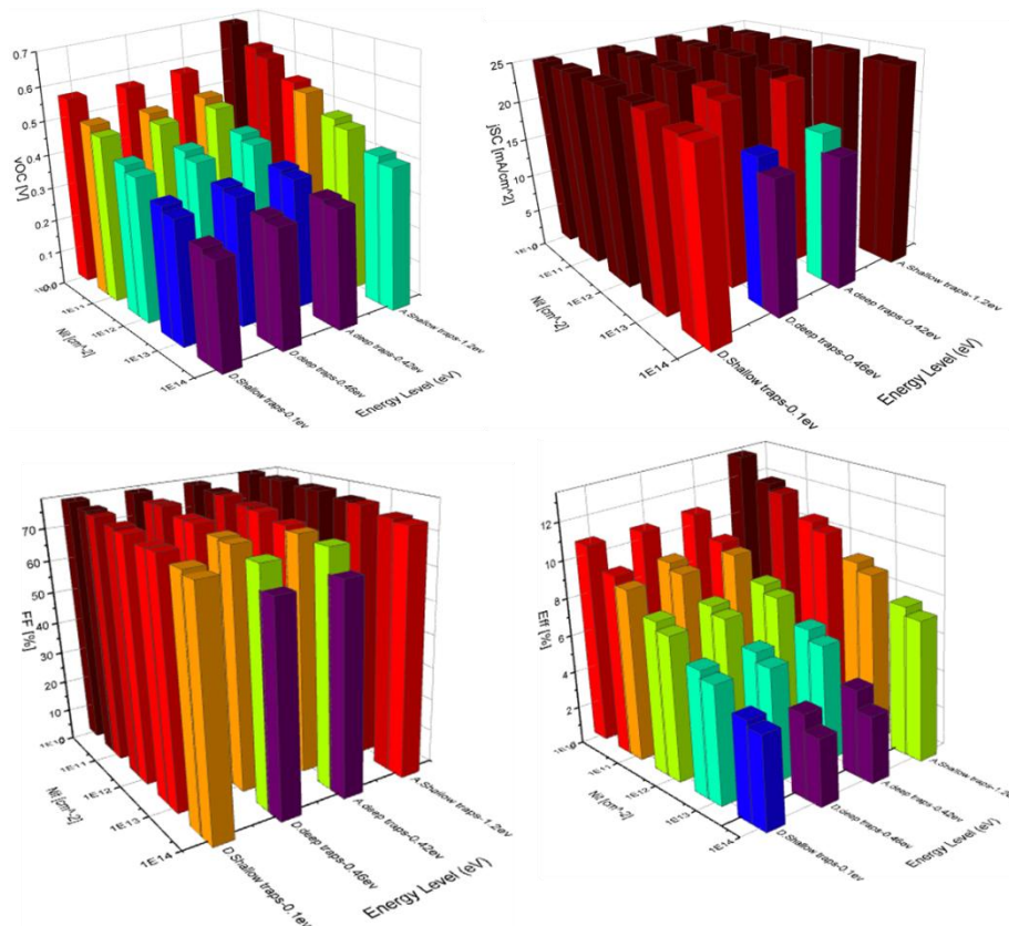
Fig. 2: shows the effect of the location of the energy states and the density of the interface states on the performance of the solar cell, all location above C.B, from 0.1ev to 1.2ev
