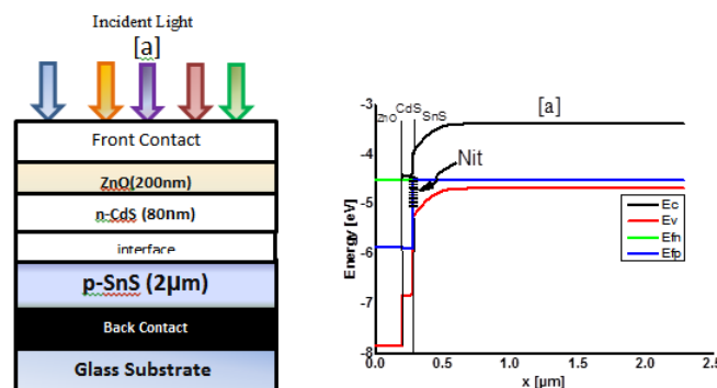
Fig. 1: shows (a) the solar cell structure and (b) the band diagram at equilibrium
