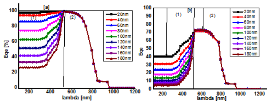
Figure (8) shows the change of quantum efficiency at the density of the interface states [a] 1E10cm^{-2} and [b] 1E14cm^{-2} with the change in the thickness of CdS.
