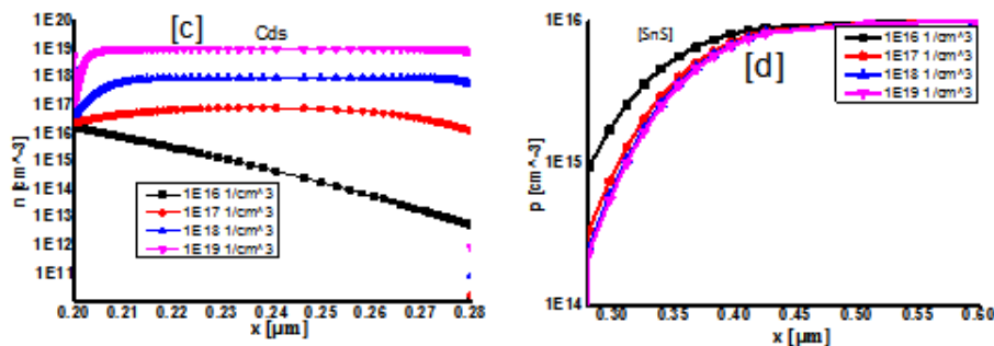
Fig. 12: illustrates the change of [a] the quantum efficiency at the density of interface defects of 1E10\text{cm}^{-2} and [b] the quantum efficiency at the density of interface defects of 1E14\text{cm}^{-2} , [c] and [d] the concentration of electrons and holes with changing concentration Carriers N_D
