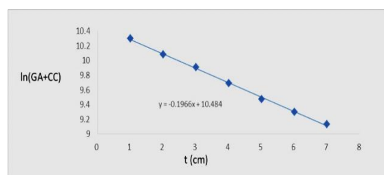
Fig. 4: Relation between \ln(GA+CC) and thickness for the mixed metallic powders material
