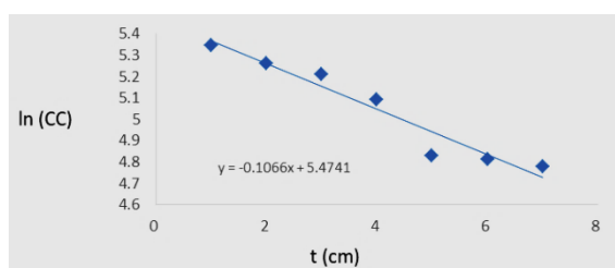
Fig. 3: Relation between \ln(CC) and thickness for the mixed metallic powders material
