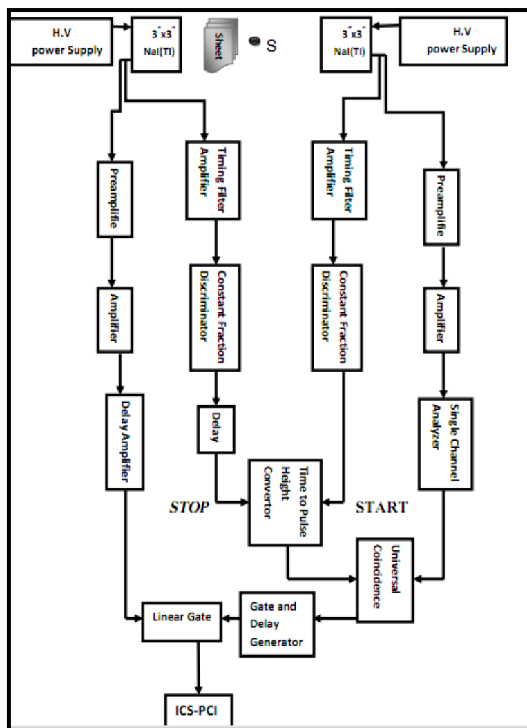
Fig. 2: Block diagram of the gamma-gamma coincidence spectrometer
