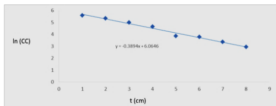
Fig. 5: Relation between ln(CC) and thickness for Fe sheets
