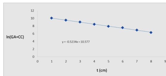
Fig. 6: Relation between ln(GA+CC) and thickness for Fe sheets
