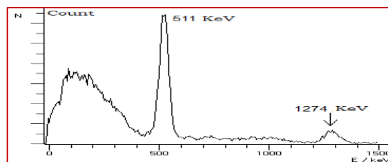
Fig 1: Typical gamma spectrum for Na-22 source obtained with NaI (TI) detector [7].
