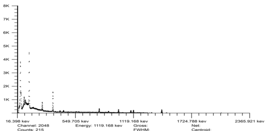
Fig. 1: Spectrum of the one-liter Marinelli beaker soil standard measured by using HpGe detector.
