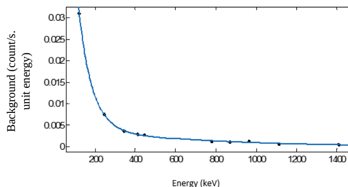
Fig. (5): Background data of Table (3) multiplied by 1.15452 and fitted by using MATLAB program.
