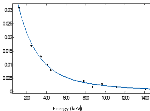
Fig. (3): Efficiency data of Table (1) fitted by MATLAB program
