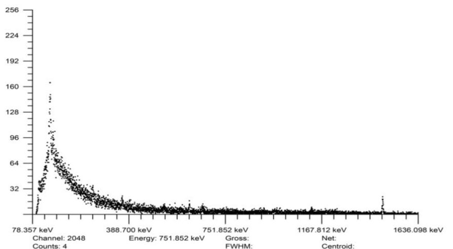
Fig. 2: Laboratory background spectrum measured by using HpGe detector.
