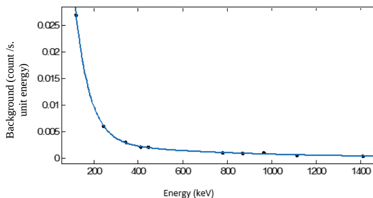
Fig. (4): Background data of Table (2) fitted by using MATLAB program.
