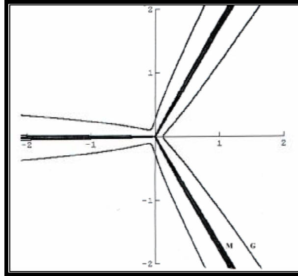
Figure (4): The thickness and the shape of the free surface for different liquids at time t = 0.1
