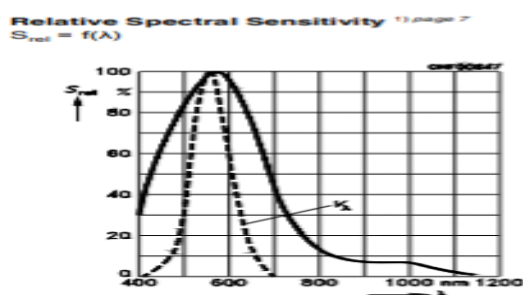
Fig. 2: shows the relationship between wavelength and sensitivity of the detector
