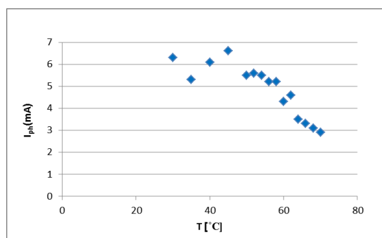
Fig. 6: shows relationship between light current and temperature by using ablu laser for adistance of one ameter
