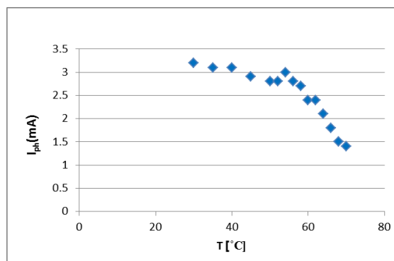
Fig. 7: shows relationship between light current and temperature by using ablu laser for adistance of one ameter and a half
