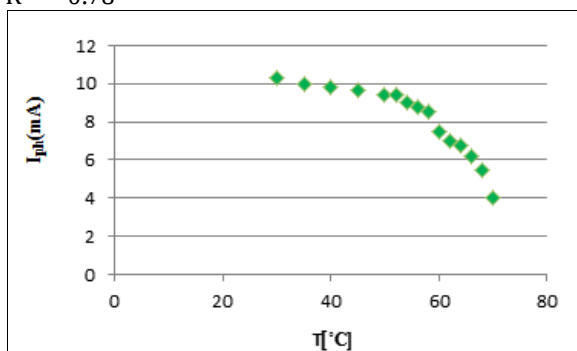
Fig. 4: shows the relationship between light current and temperature by using argon laser for adistance of two ameter
