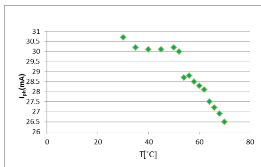
Fig. 2: shows the relationship between light current and temperature by using argon laser for adistance of one ameter
