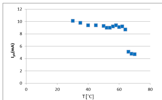
Fig. 5: shows the relationship between light current and temperature by using argon laser for adistance of half ameter
