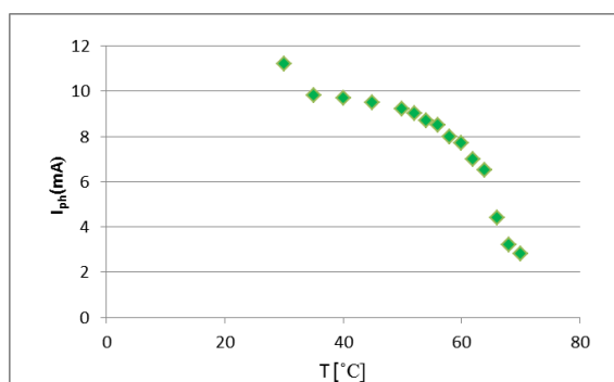
Fig. 3: shows the relationship between light current and temperature by using argon laser for adistance of one ameter and a half
