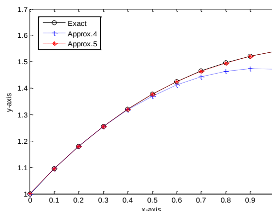
Fig. 4: Exact and Approximate Solutions for Example 4.
