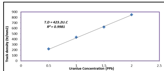
Fig .3: Pathway density and uranium concentration (ppb) for standard blood samples
