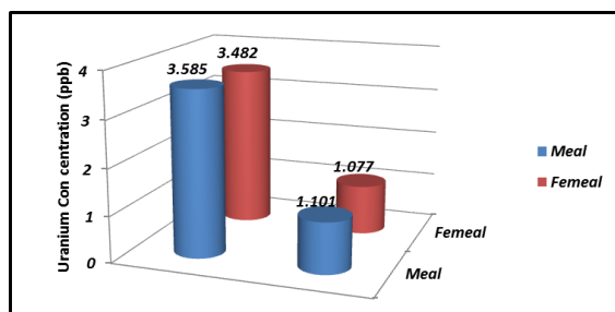
Fig.5: Uranium concentration of blood samples from Patients with cancer and health group as function of gender.
