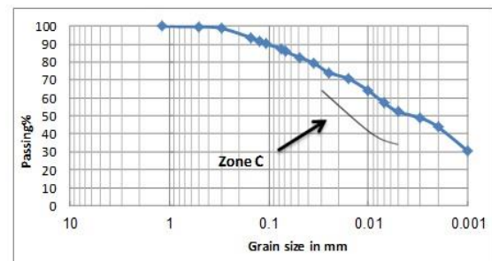
Fig. 3: Granular size analysis for the station (1).
