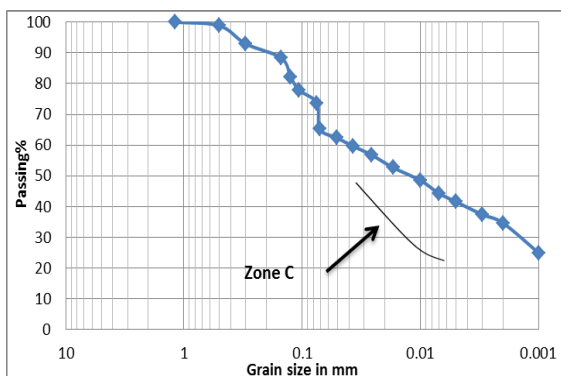
Fig. 6: Granular size analysis for the station (4).
