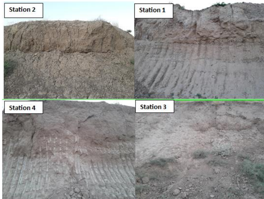
Fig. 2: The sediments stations of the study area
