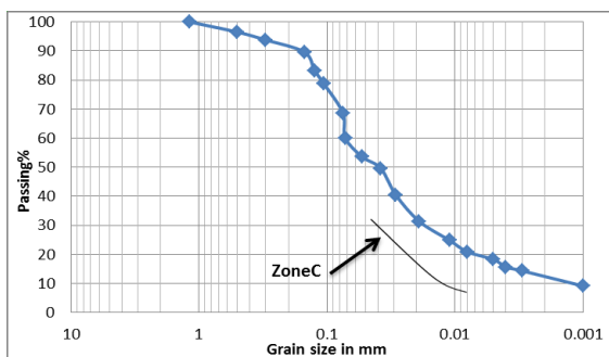
Fig. 5: Granular size analysis for the station (3).
