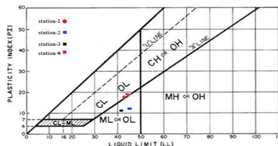
Fig. 7: Classification of the study area stations samples according to the Unified Classification
