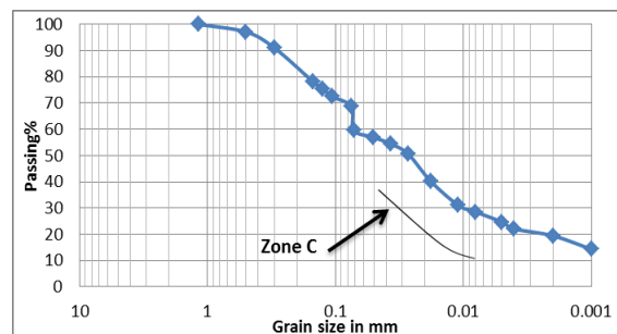
Fig. 4: Granular size analysis for the station (2).
