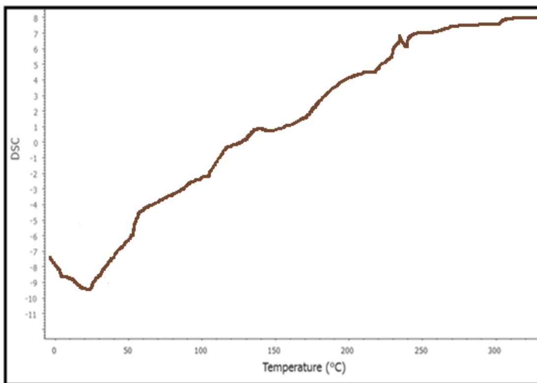
Fig (7) : DSC of Compound { 7 }
