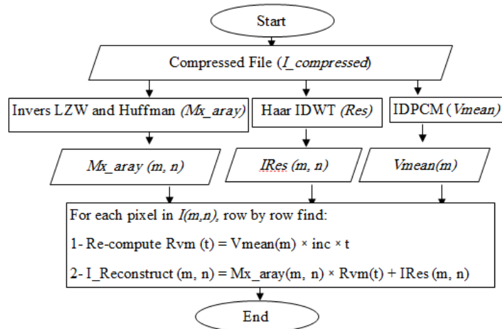
Fig. 2: Flowchart of Decoder unit
