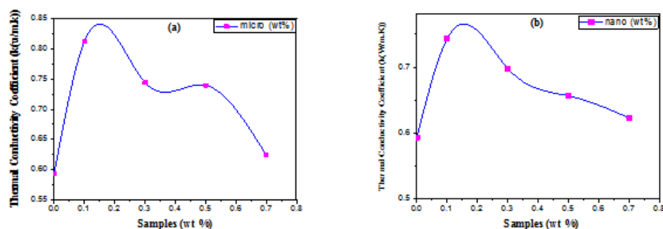
Fig. 5: shows relationship between the thermal conductivity coefficient and the different ratio of (a) micro and (b) nanoparticles of ZnO.
