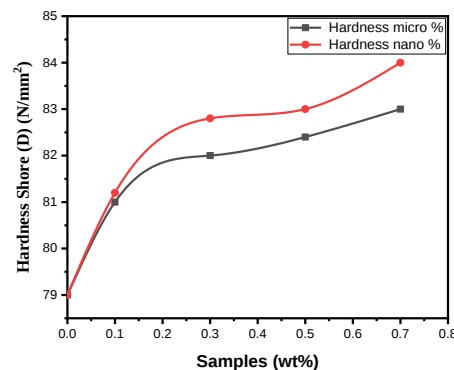
Fig. 3 shows relationship between the hardness values and the different ratio of micro and nanoparticles of ZnO.
