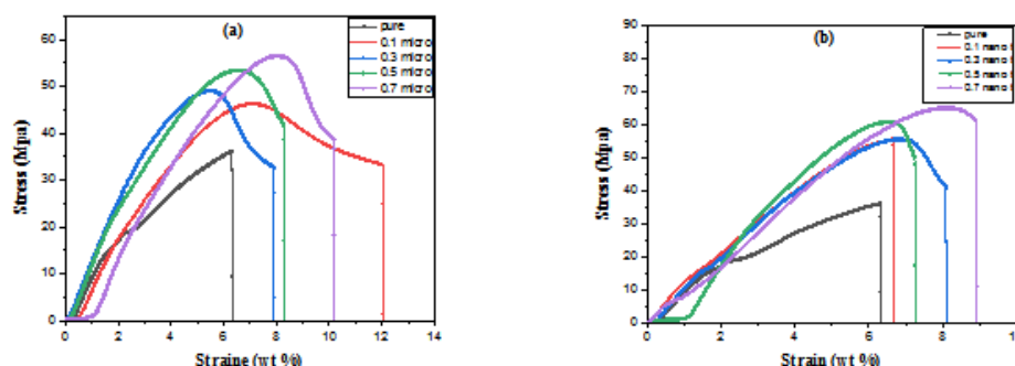
Fig. 1: shows the relationship between stress and strain curves for the epoxy compositions supported by (a) ZnO microparticles (b) ZnO nanoparticles.
