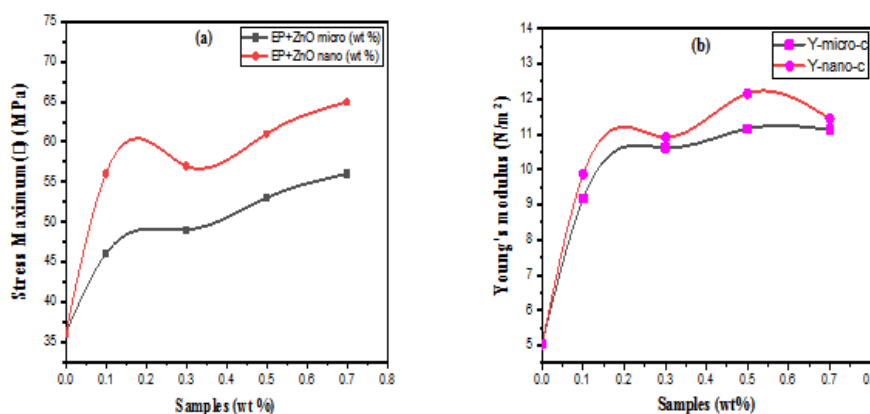
Fig. 2: shows the relationship between (a) the highest tensile stress value (b) Young's modulus and the different ratio of micro and nanoparticles of ZnO.
