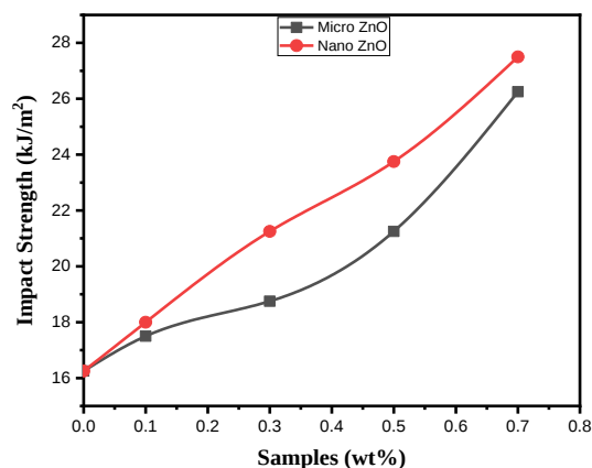
Fig. 4: shows relationship between the shock test values and the different ratio of micro and nanoparticles of ZnO.
