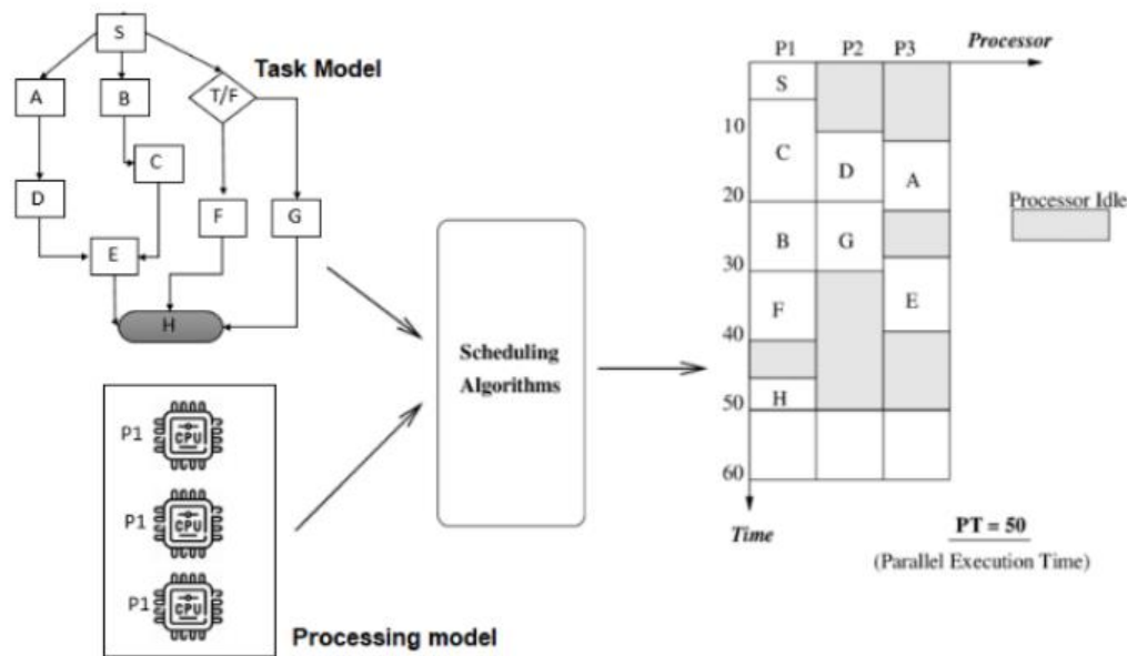
Figure 4. Task scheduling example [27]
