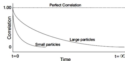
Fig. 1: shows the relationship between communication functions for large and small particles show.
