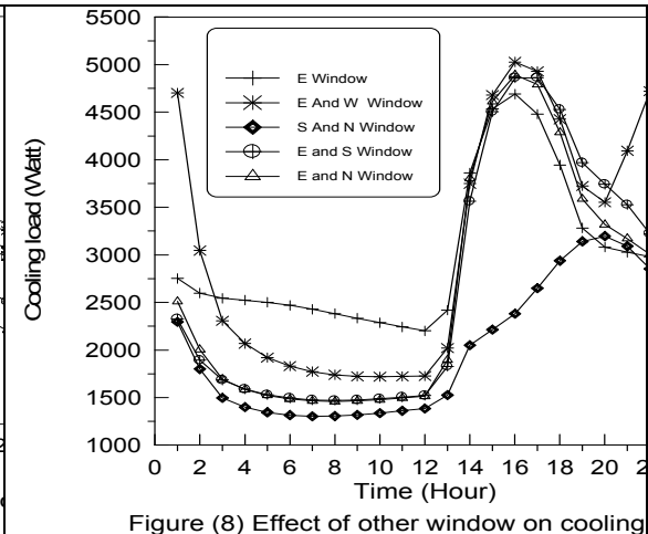
Figure (8) Effect of other window on cooling load
