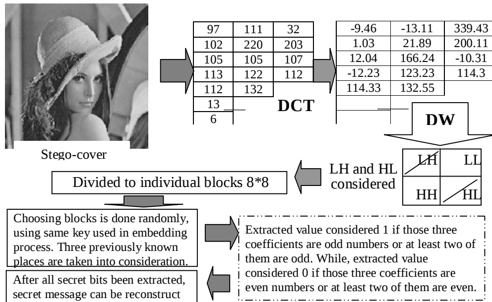
Figure (13): Recovery process of DCT+DWT method
