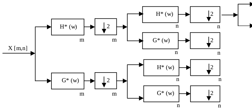
Figure (3): Two-Dimensional DWT.
