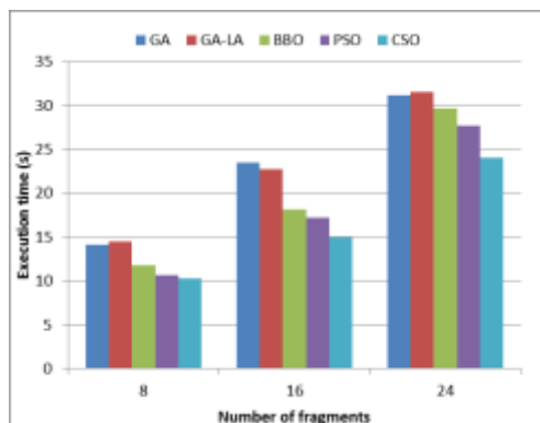
Fig. 6: Execution time for 8 sites
