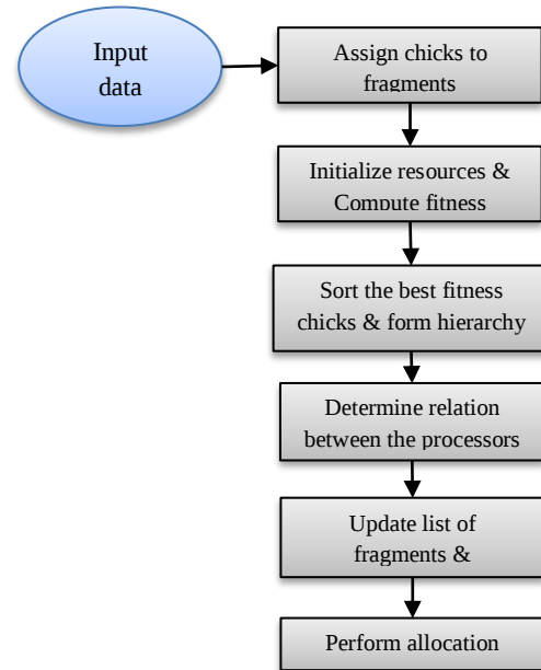
Fig. 2: CSO based DAP approach
