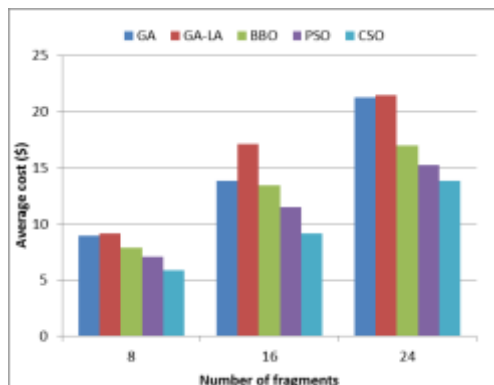
Fig. 5: Average cost for 8 sites
