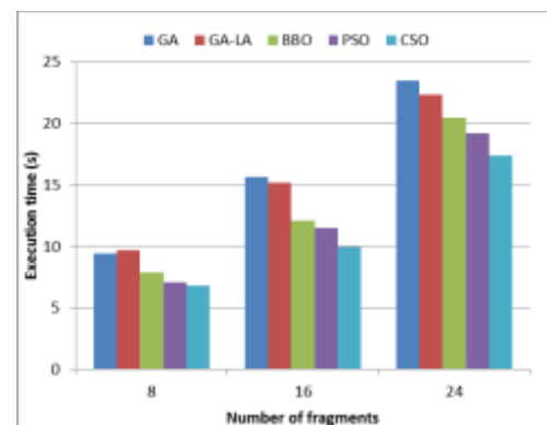
Fig. 4: Execution time for 4 sites
