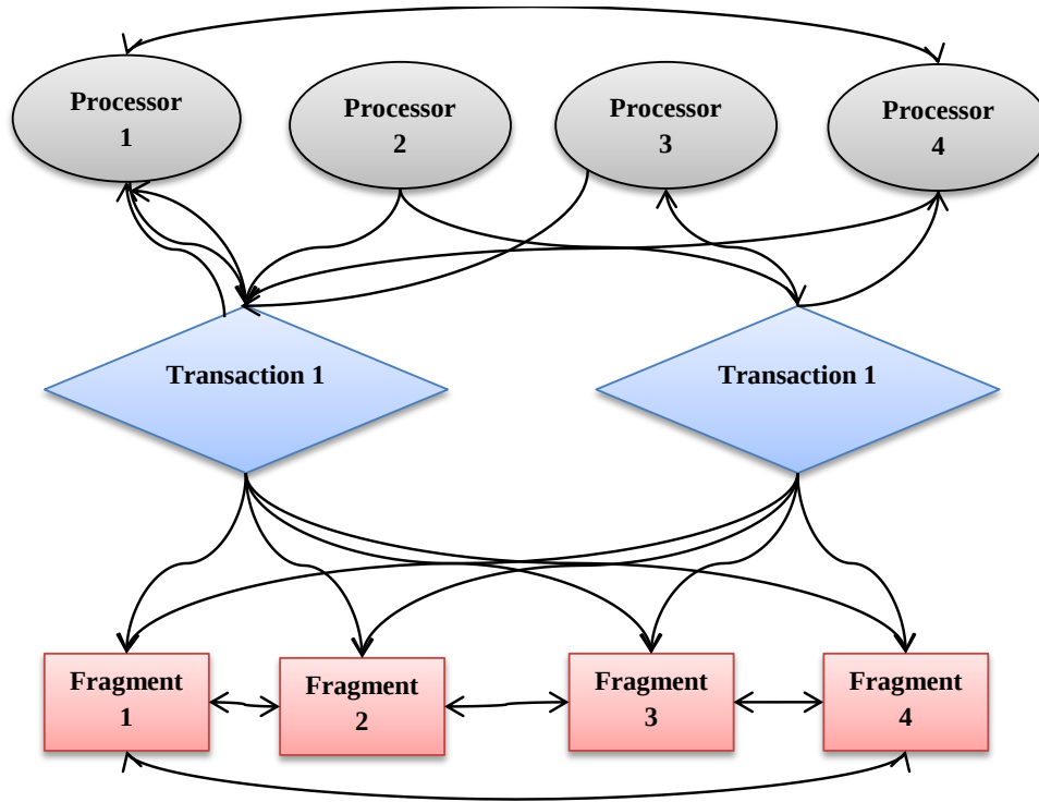
Fig. 1: Dependencies of transactions on fragments and processors on transactions
