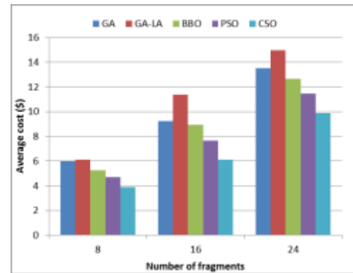
Fig. 3: Average cost for 4 sites
