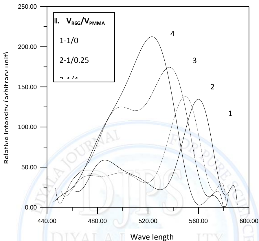
Figure (5) absorption spectra for rhodamine 6G in \text{CHCl}_3
