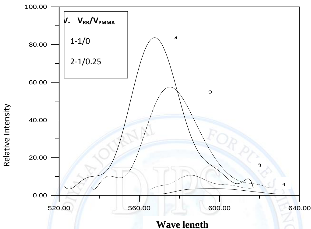
Figure (3) florescence spectra for rhodamine B in \text{CHCl}_3
