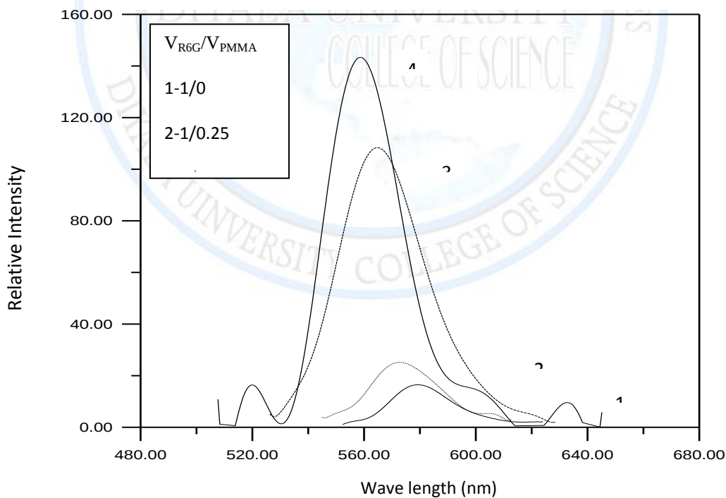
Figure (8) florescence spectra for rhodamine 6G in \text{CH}_3\text{OH}
