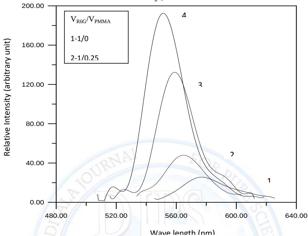
Figure (7) florescence spectra for rhodamine 6G in \text{CHCl}_3
