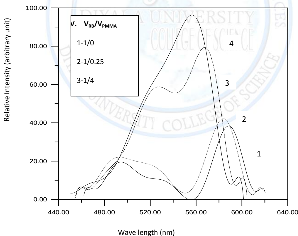
Figure (1) absorption spectra for rhodamine B in \text{CHCl}_3
