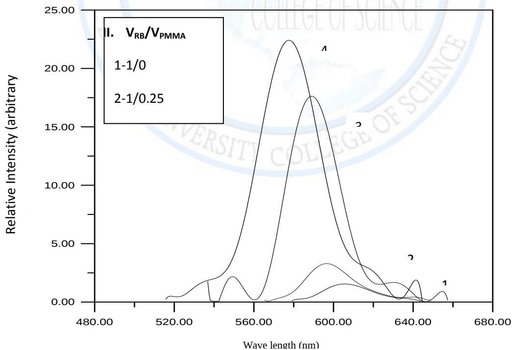
Figure (4) florescence spectra for rhodamine B in \text{CH}_3\text{OH}
