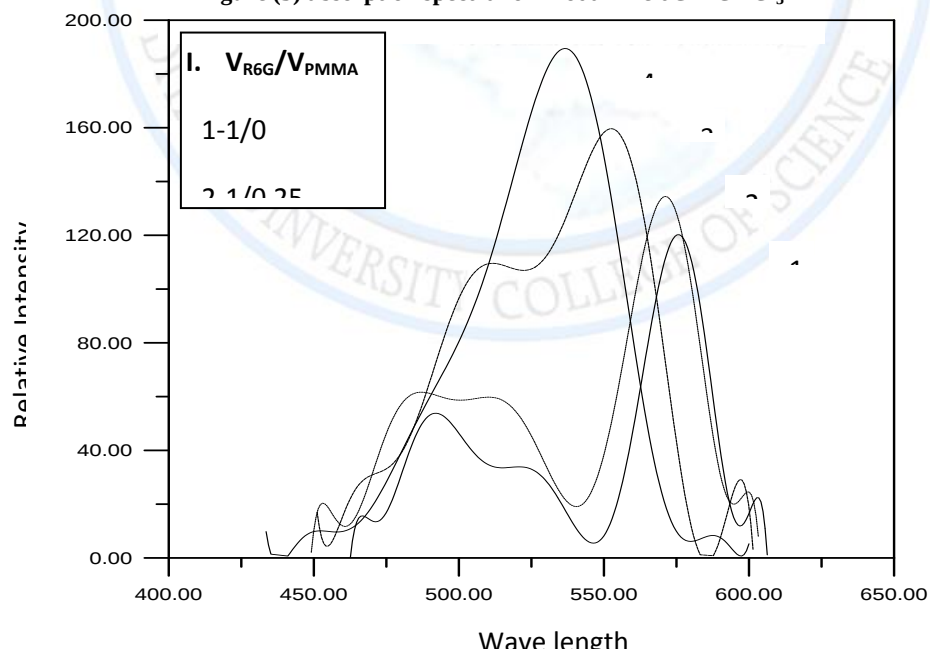
Figure (6) absorption spectra for rhodamine 6G in \text{CH}_3\text{OH}
