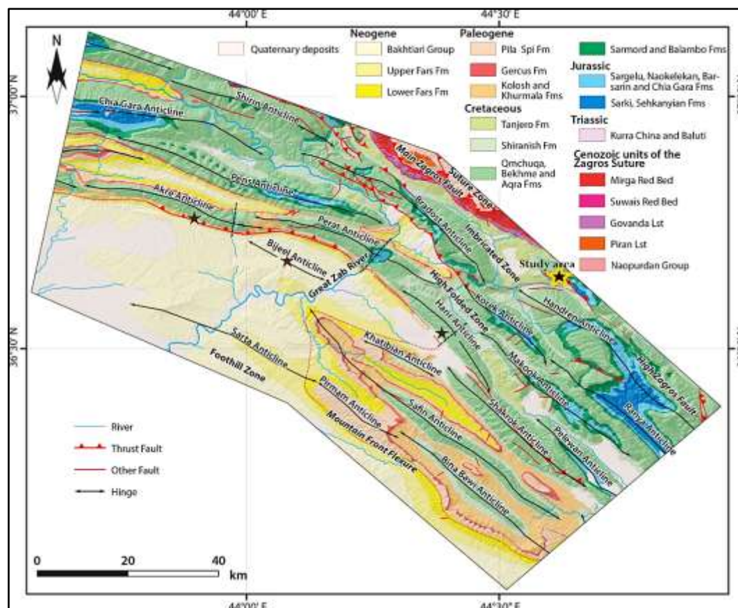
Fig. 2: Geological map of the Imbrication Zone, NE-Iraq (modified after Csonotos et al., 2012; Zebari and Burberry, 2015).
