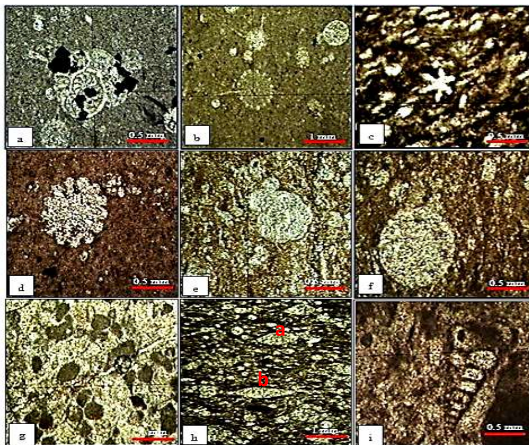
Fig. 7: Carbonate petrographic component; a) Larva- ammonite partially replaced by cubic pyrite, Ch11, P.L. b) Radiolaria within micritic matrix. Ch1, P.L. c) Sponge spicules (Hexactine), Ch112, P.L, A.S. d) Echinoid spine within micritic matrix, Ch36, P.L, A.S. e) Ticinella sp (Planktonic foraminifera) within neomorphosed micritic matrix, Ch89, P.L. f) Unwalled calcisphere in micritic matrix, Ch63, P.L, A.S.g) Fecal peloids in neomorphosed micritic matrix, Ch58, P.L.h) (a) articulate ostracods and (b) Pelecypods within micritic matrix, Ch40. i) Textularian (Benthic foraminifera with micrite envelope, within micritic matrix, Ch41, P.L, A.S. Key: Ch, Chombarok; P.L., Plain polarized, A.S., Alizarin stained.
