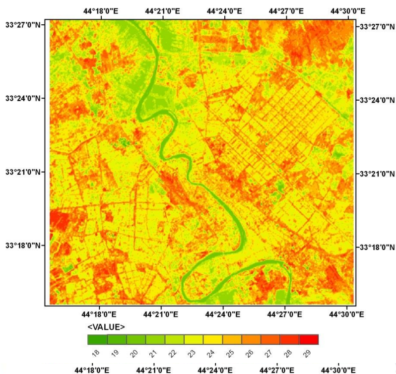
Figure 7: LST map of the study area.
