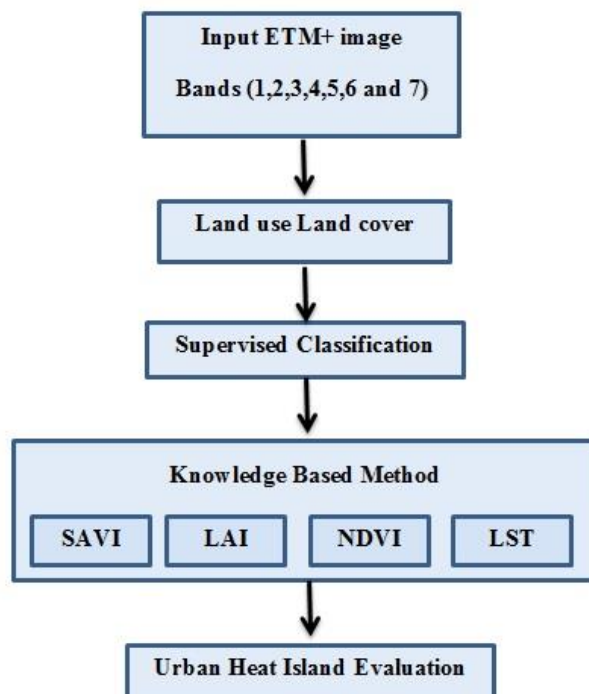
Figure 2: Flow chart of evaluation of urban heat island from Landsat 7 ETM+ image for the study area
