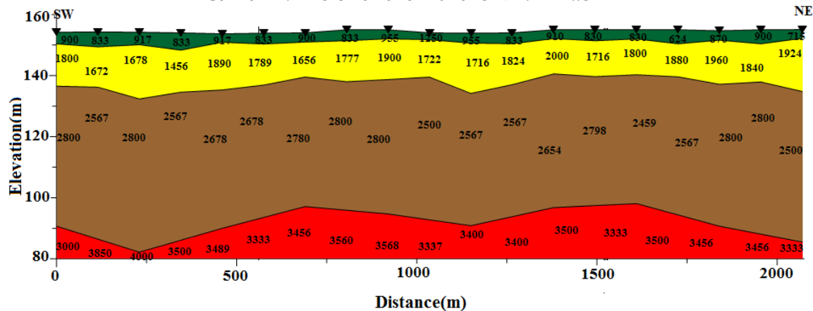
Figure (6) Seismic section at the left bank of Euphrates river
