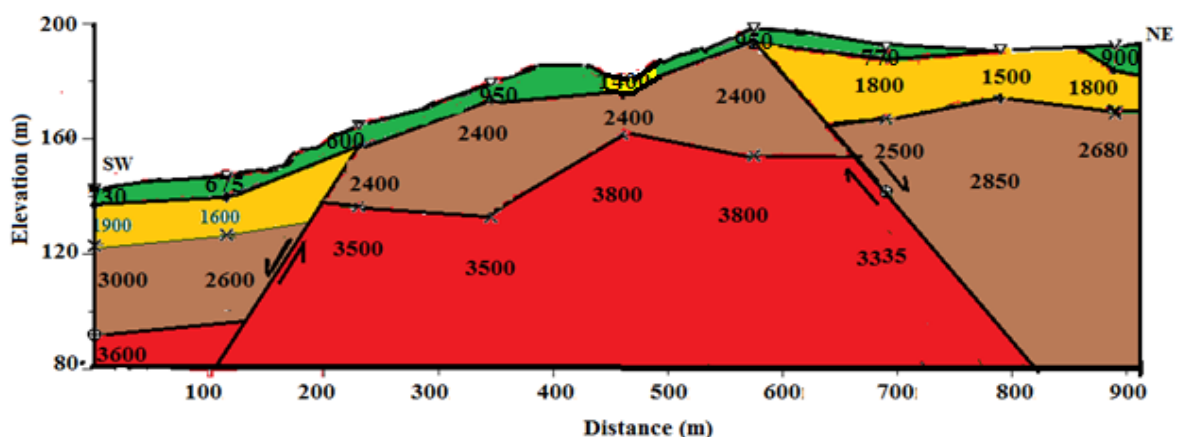
Figure (5) seismic section at the right bank of Euphrates River
