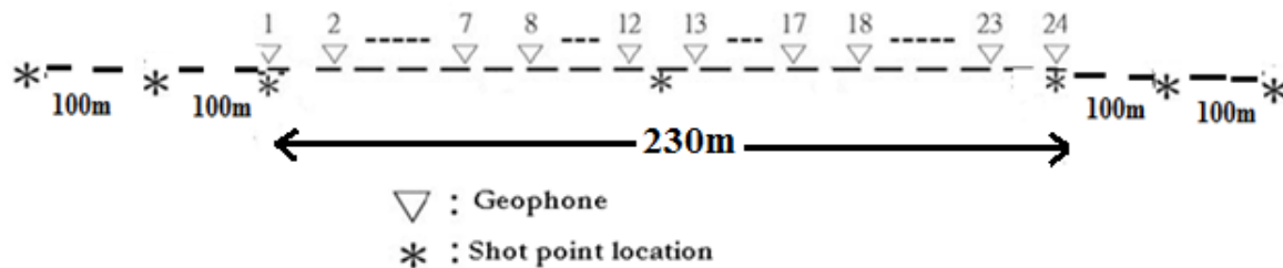
Figure (3) Geophones distribution and shot points locations
