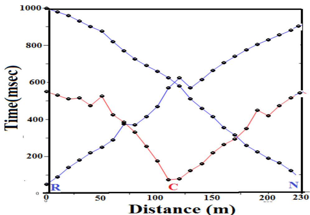
Figure (4) Time distance graph for spread 2 at right bank area with out offsets
