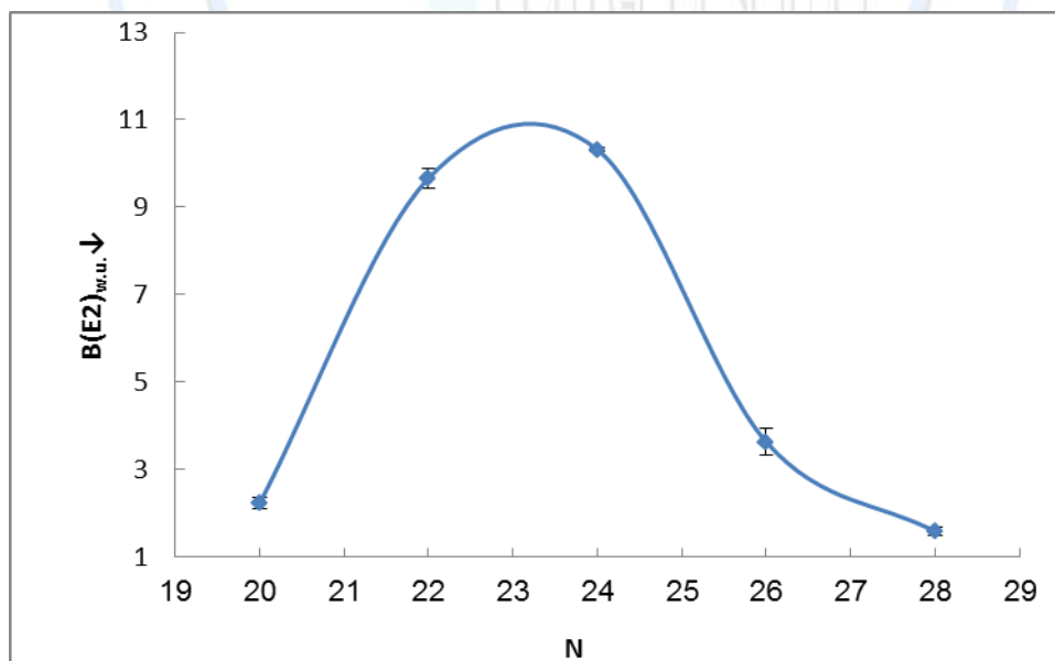
Figure -2: Reduced transition probability B(E2)_{w.u.} , for \gamma_0 - transitions as a function of the neutron number in ^{20}\text{Ca} nuclei.
