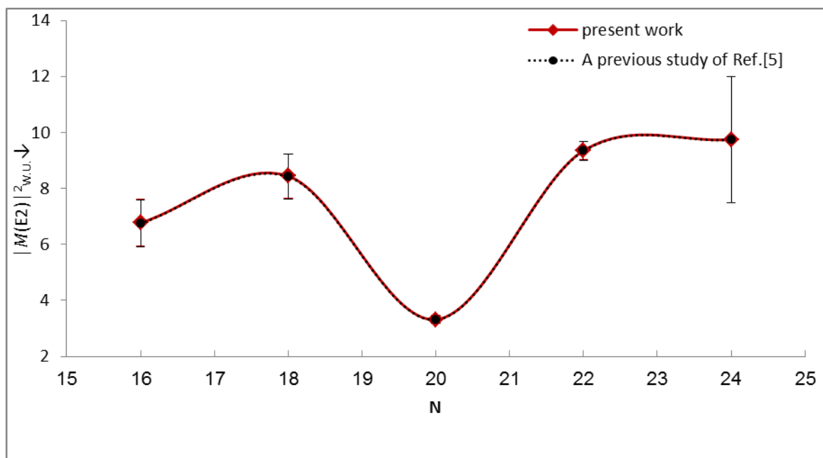
Figure -3: Comparison between the [M(E2)]^2_{w.u.} values of the present work for ^{18}\text{Ar} nuclei with other study of ref.[5].
