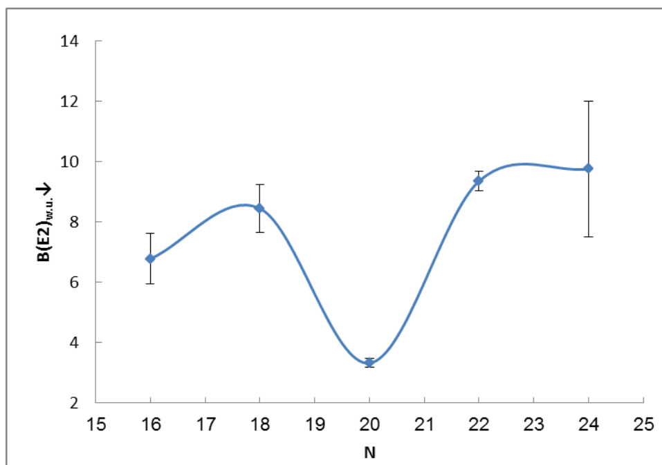
Figure -1: Reduced transition probability B(E2)_{w.u.} , for \gamma_0 - transitions as a function of the neutron number in ^{18}\text{Ar} nuclei.
