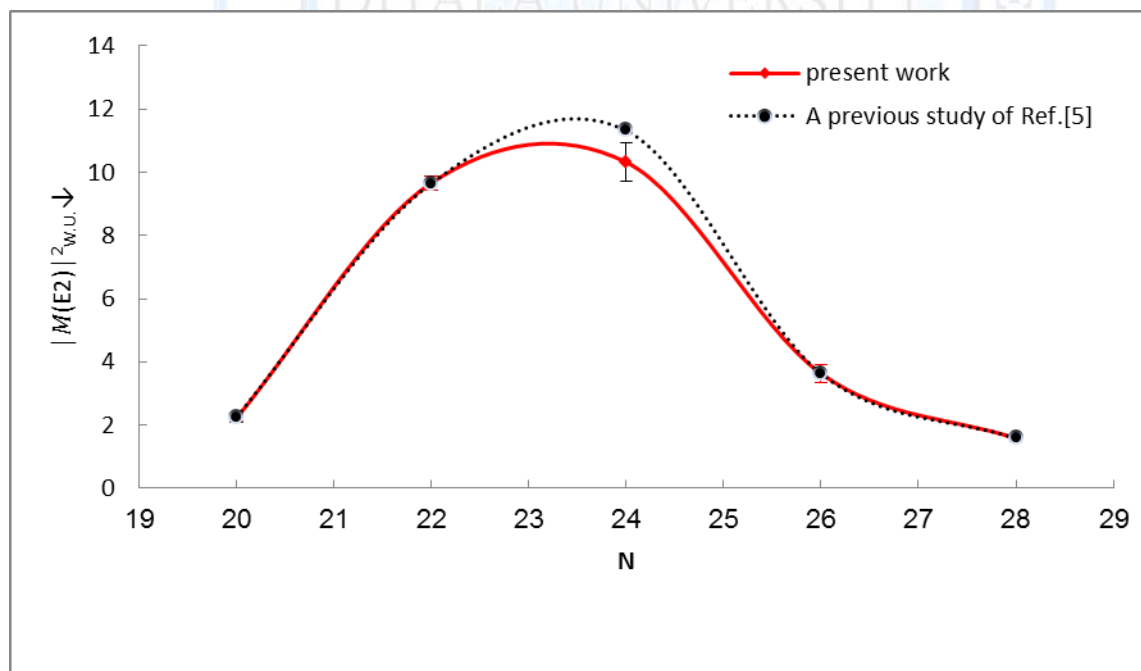
Figure -4: Comparison between the [M(E2)]^2_{w.u.} values of the present work for ^{20}\text{Ca} nuclei with other study of ref.[5].
