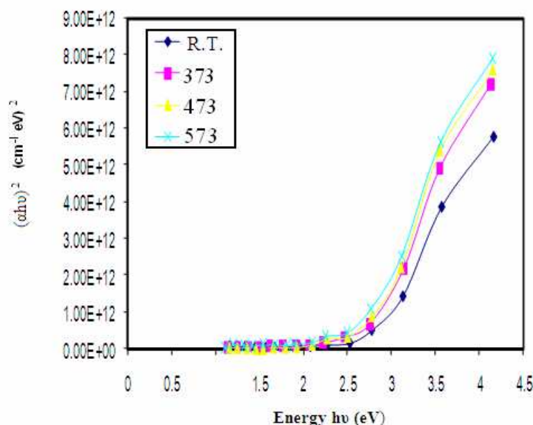
Fig.(2) (\alpha h\nu)^2 vs. h\nu plot for CdTe thin films deposited at R.T. and annealed with different temperatures.
