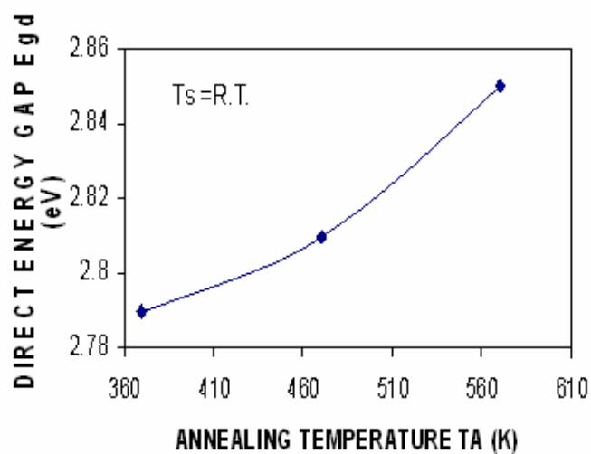
Fig.(4): The allowed direct energy gap E_{gd} vs. annealing temperature T_A for CdTe thin films deposited at R.T.
