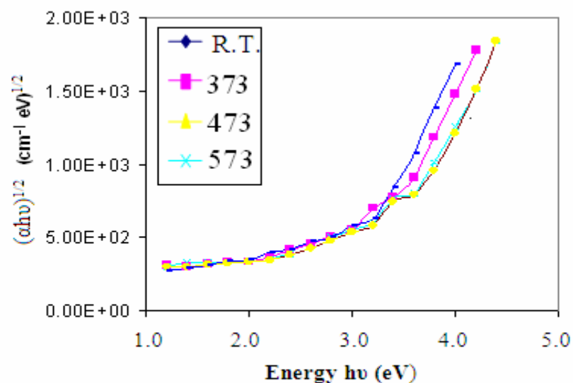
Fig.(3) (\alpha h\nu)^{1/2} vs. h\nu plot for CdTe thin films deposited at R.T. and annealed with different temperatures.
