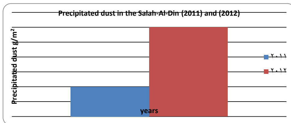
Fig (10) Precipitated dust quantities (annual rate) in the Salah-Al-Din (2011) and (2012)
