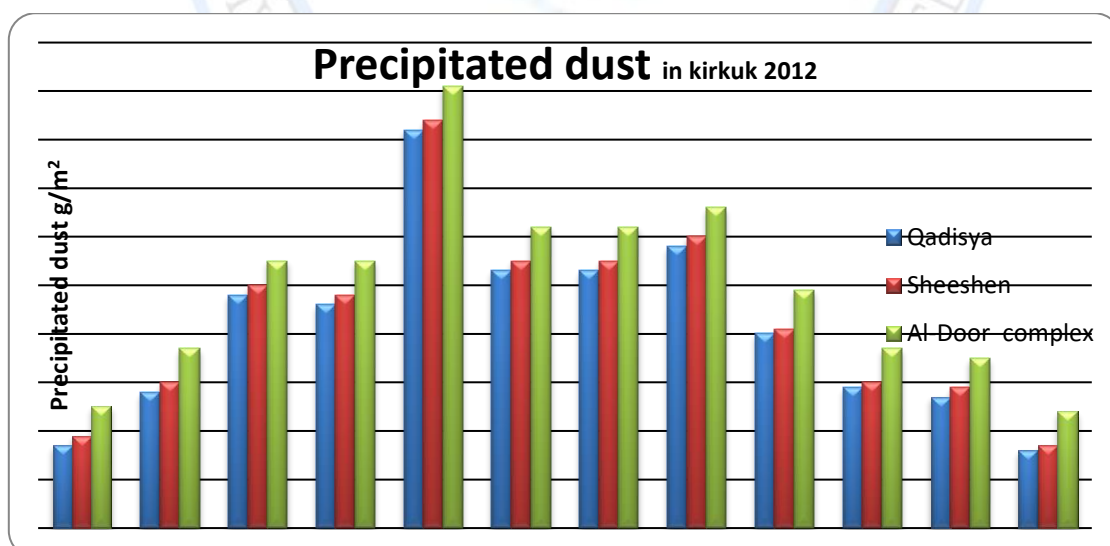
Fig (3) Precipitated dust amounts in Kirkuk, 2012
