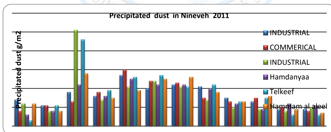
Fig (11) Precipitated dust quantities (annual rate) in Nineveh for the year (2011)
