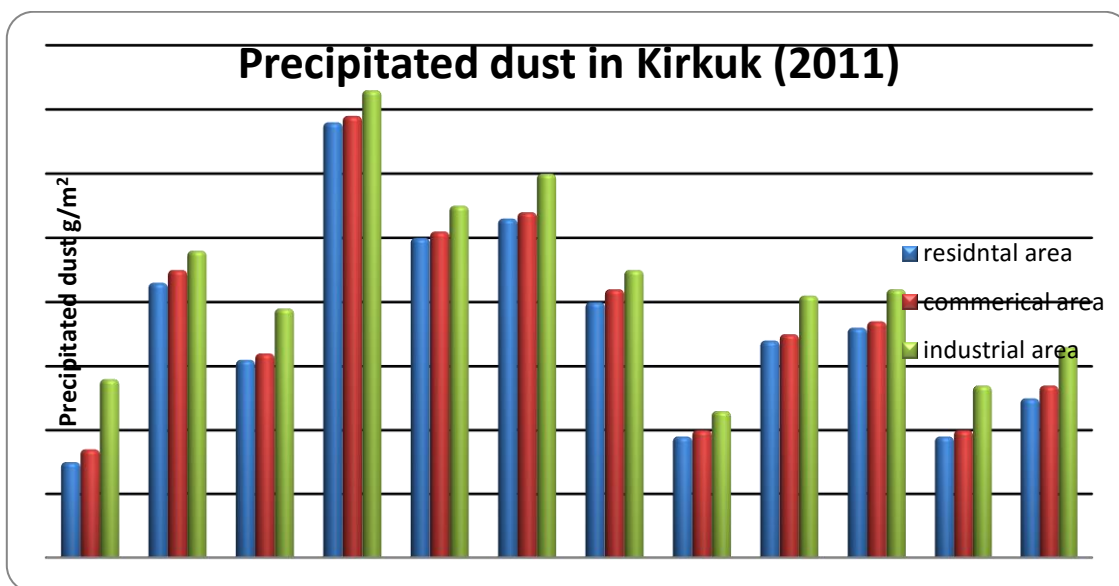
Fig (2) Precipitated dust amounts in Kirkuk (2011)
