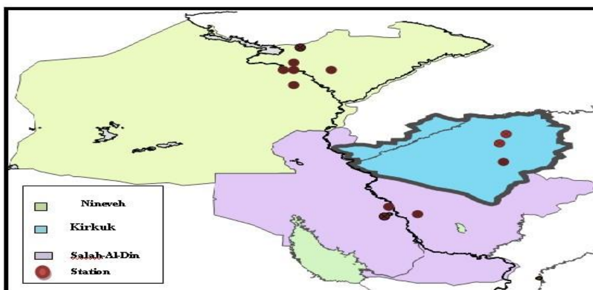
Figure (1) location of stations at study area
