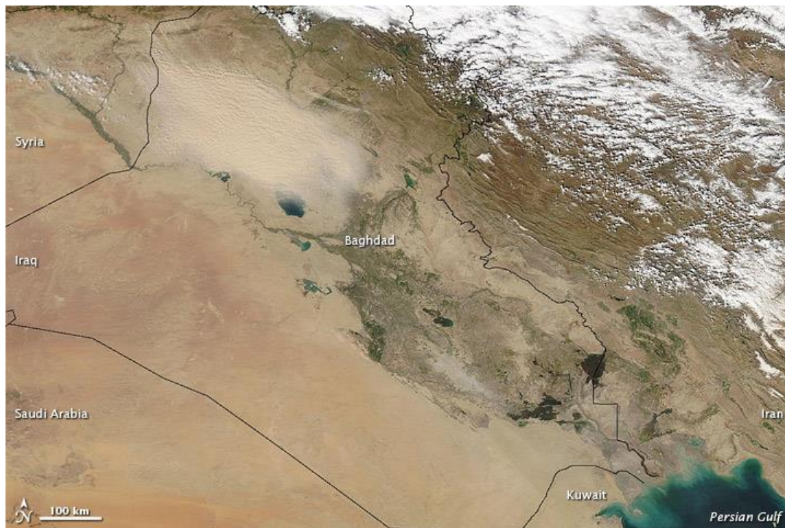
Fig (12) Dust Storm over Iraq March 3, 2011
