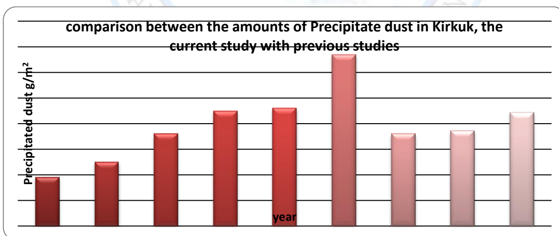
Fig (5) a comparison between the amounts of precipitated dust in Kirkuk, the current study with previous studies
