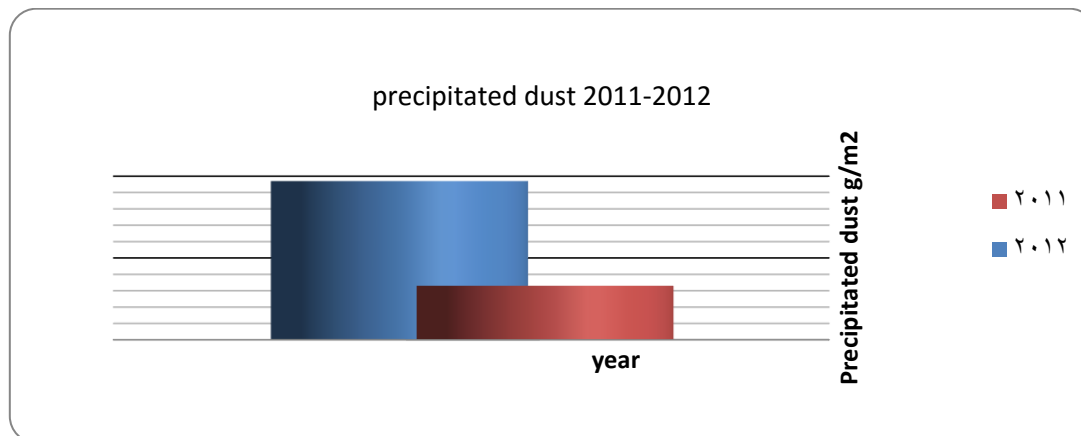
Fig (4) Precipitated dust quantities (annual rate) in Kirkuk for the years (2011) and (2012)
