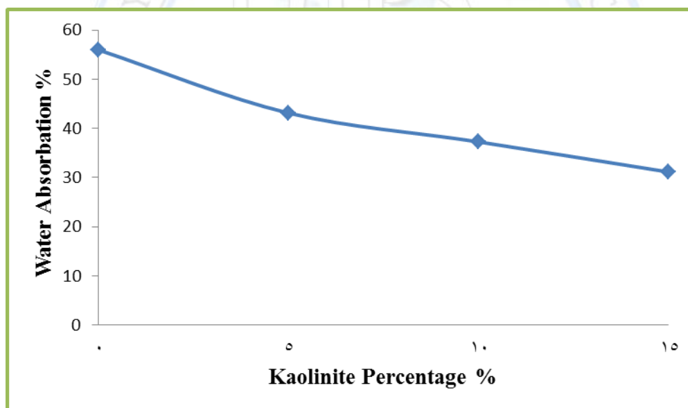
Figure (8): Effect of kaolinite percentage additions on water absorption.
