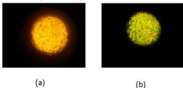
Fig. 4: The wafer of p-type silicon with amplification by 600 times for the internal composition of the (a) before the thermal oxidation (b) after cleaning and thermal oxidation with maximum temperature ( 1200^{\circ}\text{C} ).
