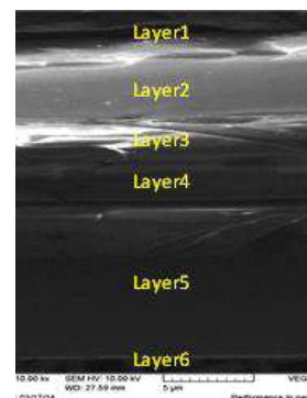
Fig. 14: Cross - sectional scanning electron microscopy (SEM) images for the device with CuO coating.
