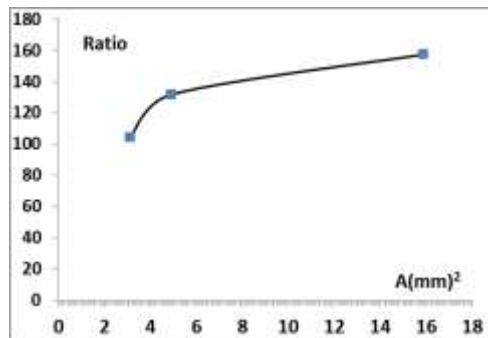
Fig. 10: The relation between A and R_{ratio} for the device with CuO coating.
