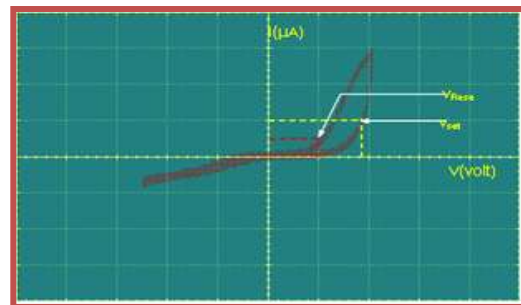
Fig. 13: The AC measurements of the device with CuO coating in case of .
