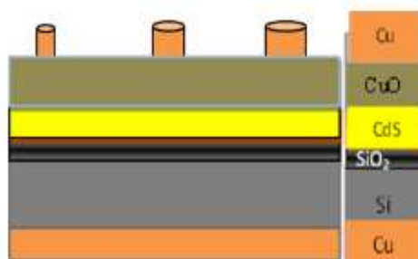
Fig. 7: The cross section of the structures.
