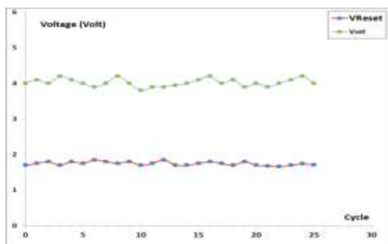
Fig. 12: Endurance of the voltages ( V_{set} and V_{Reset} ) of the device with CuO coating in case of TEL.
