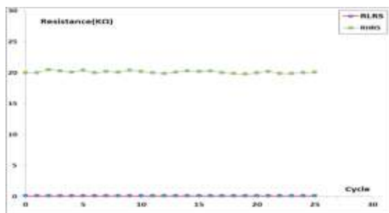
Fig. 11: Endurance for resistance LRS and HRS of the device with CuO coating in case of TEL.
