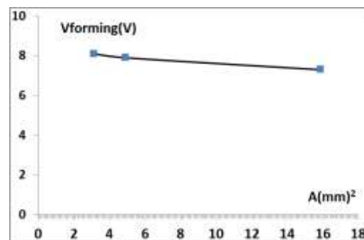
Fig. 9: The relation between A and V_{\text{forming}} for many devices with CuO coating.
