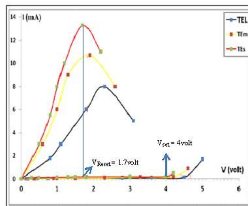
Fig. 8: (I-V) properties for the device with CuO coating for many electrodes areas using compliance current I_{cc}=20\text{mA} .
