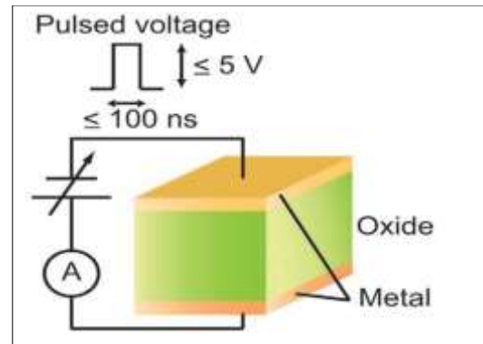
Fig. 1: Diagram of a ReRAM memory cell with a capacitor-like structure in which an insulating or semiconducting oxide is sandwiched between two metal electrodes[6]
