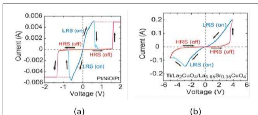
Fig.2: I - V curves during different type of resistive switching: (a) unipolar switching in a Pt/NiO/Pt cell and (b) bipolar switching in a Ti/La 2 CuO 4 /La 1.65 Sr 0.35 CuO 4 cell. [9].
