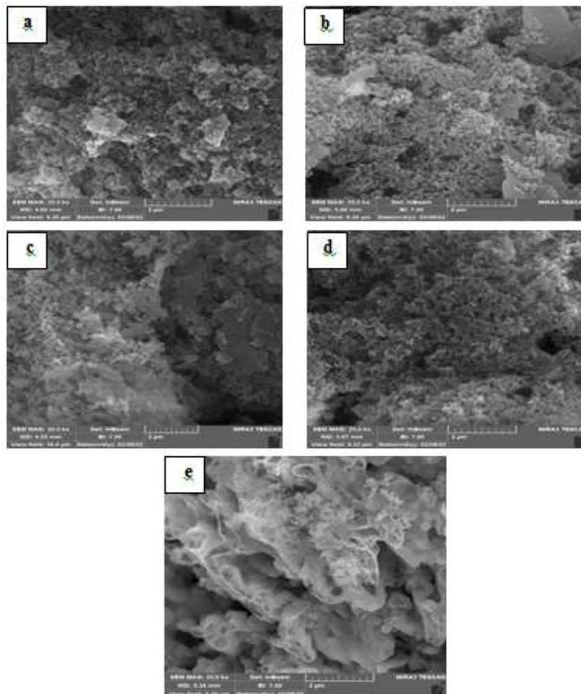
Fig. 6: SEM images of the Cermet Composites (Ni-5%Al 2 O 3 -% B_4C ) Where: (a) 5% B_4C , (b) 10% B_4C , (c) 15% B_4C , (d) 20% B_4C , (e) 25% B_4C
